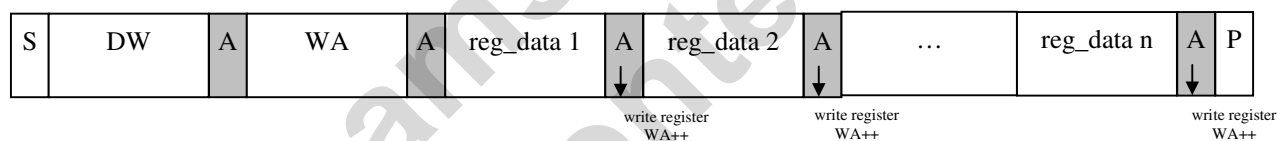
Figure 2 – I^2C Page-Write:
