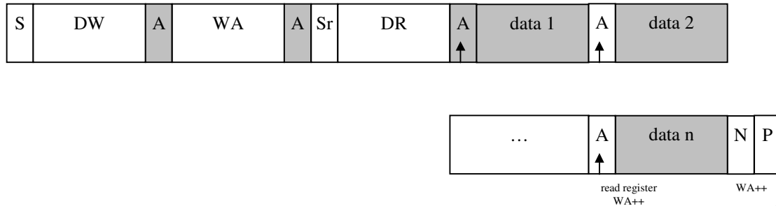
Figure 4 – I^2C Sequential-Read:
