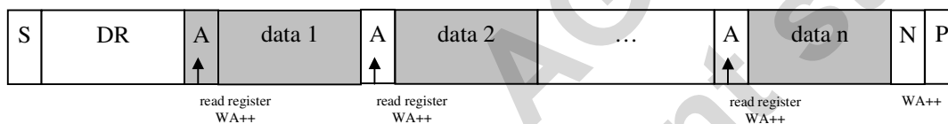
Figure 5 – I^2C Current-Address-Read:
