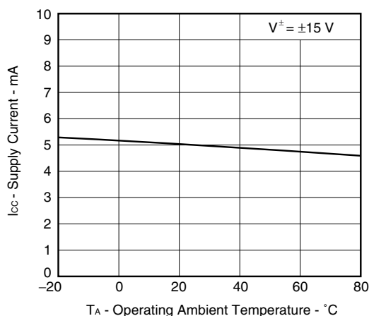
SUPPLY CURRENT
