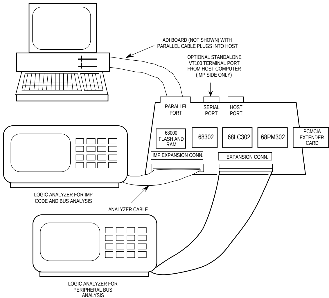
Figure 1. MC68302FADS
