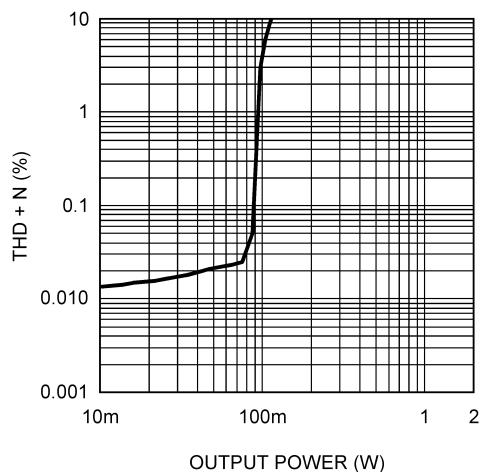
THD+N vs Output Power V_{DD} = 5V , R_L = 32\Omega , SE, f = 1kHz
