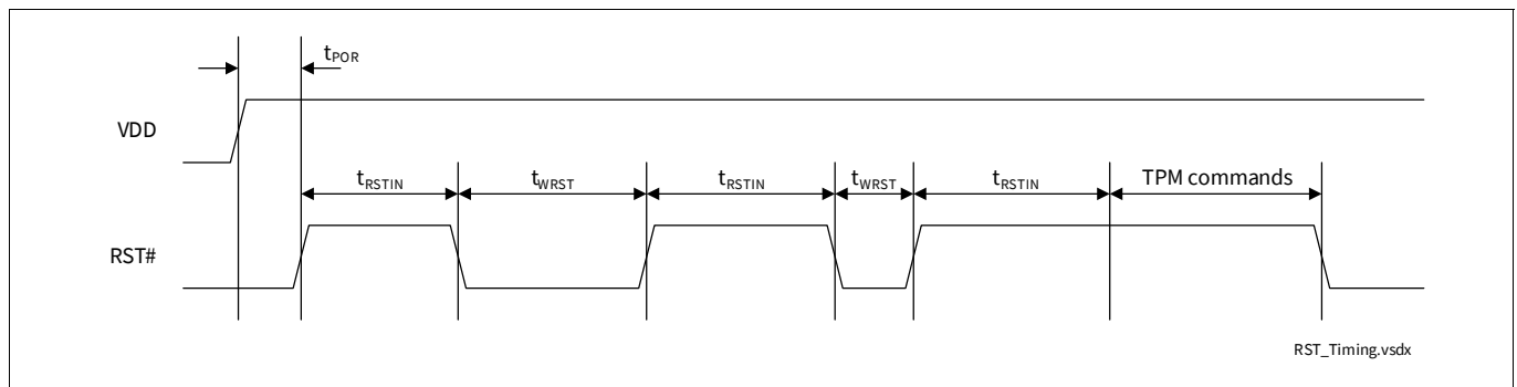
Figure 3 RST# Timing
