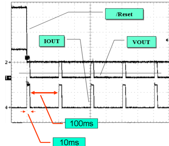
Figure 14. Switching Converter Over-current Protection
