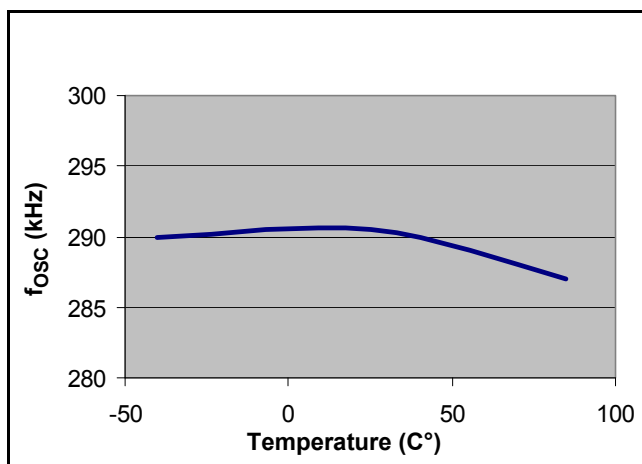
Figure 5. f_{\text{OSC}} vs. Temperature
