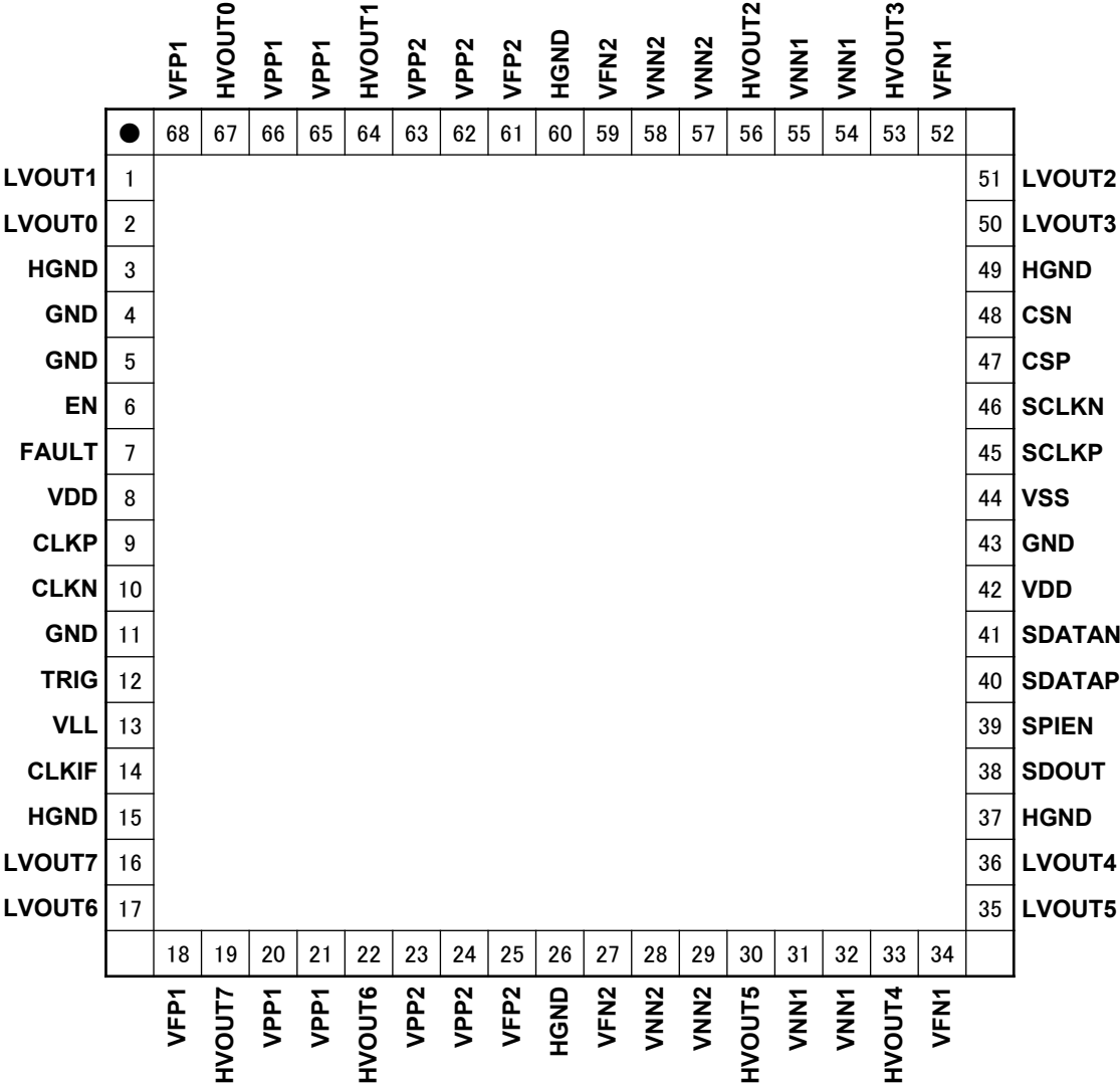
Figure 16 Pin Configuration
