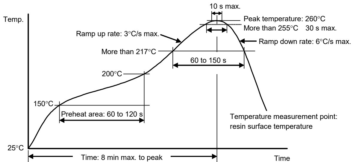
Figure 17 Resistance to soldering heat condition for package (Reflow method)
