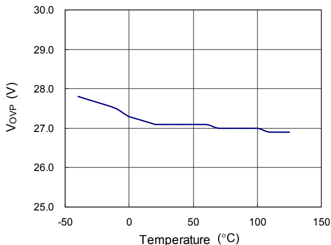
Over Voltage Protection Level ( V_{OVP} ) vs. Temperature
