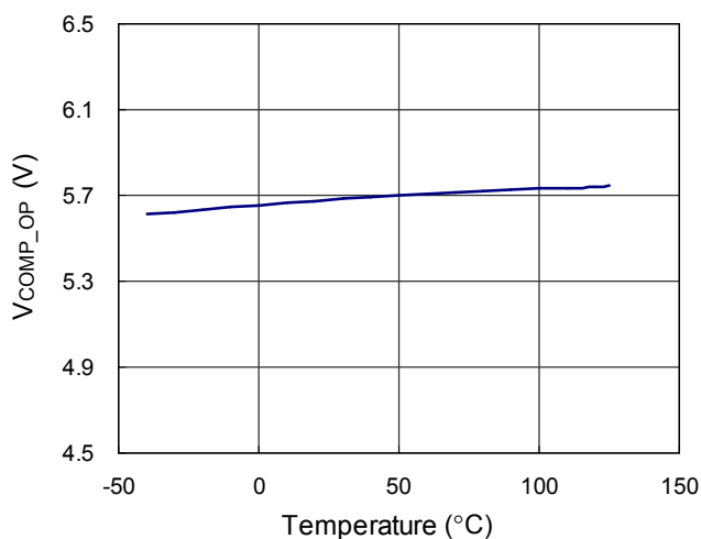
Comp Open Voltage ( V_{COMP\_OP} ) vs. Temperature
