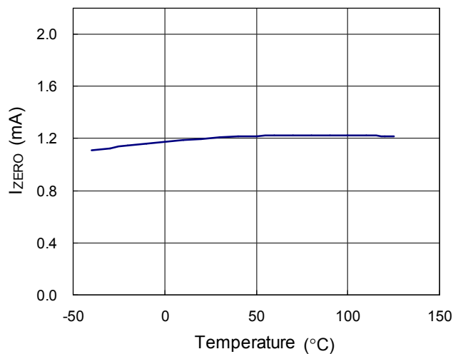
Comp Short Current ( I_{ZERO} ) vs. Temperature
