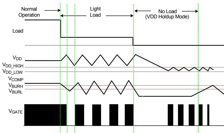
Figure 1. Burst Triple-Mode
