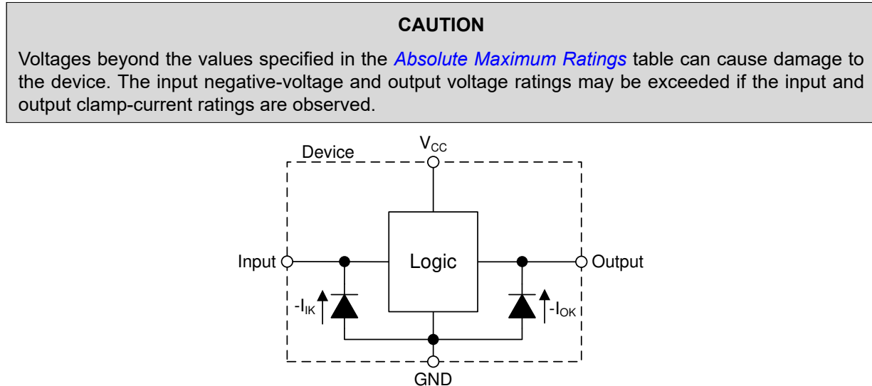
Figure 8-1. Electrical Placement of Clamping Diodes for Each Input and Output
