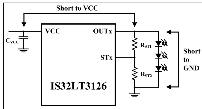
Figure 35 OUTx Pins Short Operation
