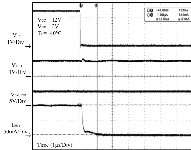
Figure 27 EN Off
