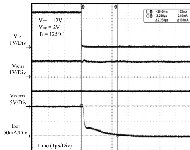
Figure 29 EN Off
