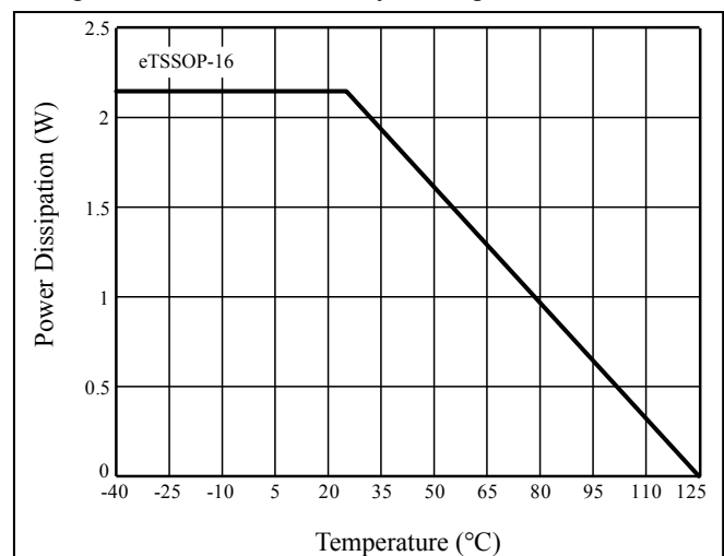
Figure 36 Dissipation Curve
