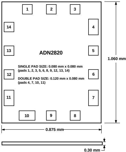
Figure 20. 14-Pad Bare Die Dimensions shown in millimeters
