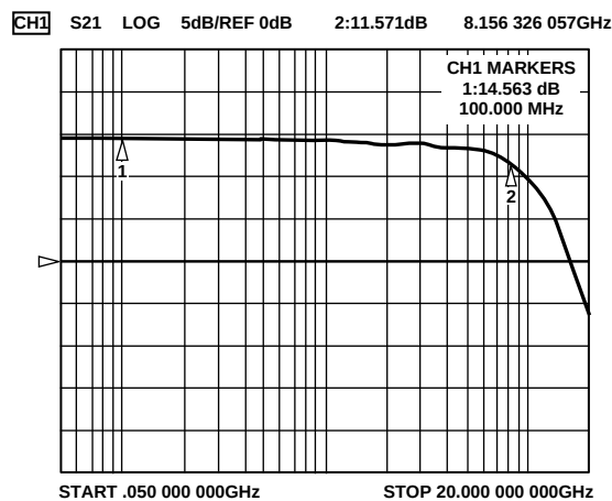
Figure 5. ADN2820 S_{21}
