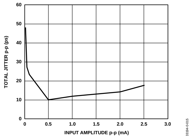
Figure 10. Total Jitter Peak-to-Peak vs. Input Amplitude ( ER = 10 \text{ dB} )
