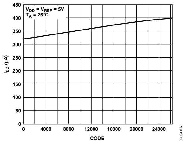
Figure 11. Supply Current vs. Code
