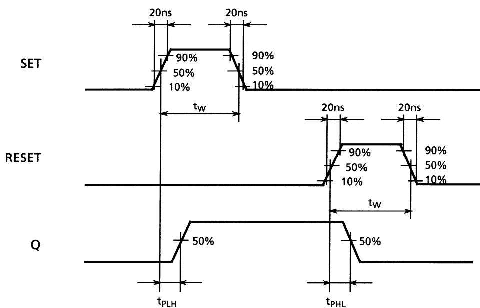
Waveform 2
