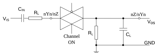
(a) Channel ON Condition
