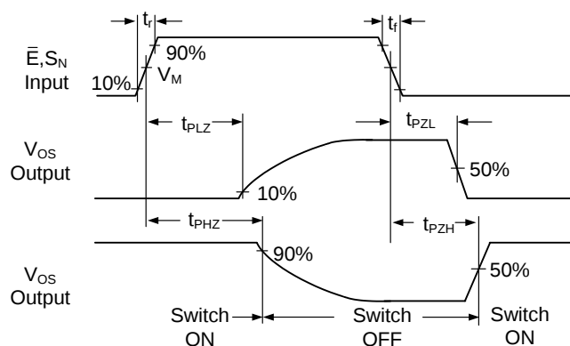
Figure 21. Waveforms Showing the Turn-on and Turn-off Times ( V_M = 50\% , V_I = \text{GND to } V_{CC} )
