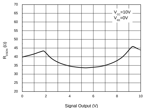
Figure 10. R_{DS(on)} vs. Signal Output
