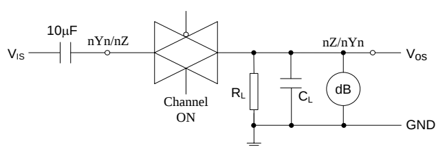
Figure 4. Test Circuit for Measuring Sine-wave Distortion and Minimum Frequency Response
