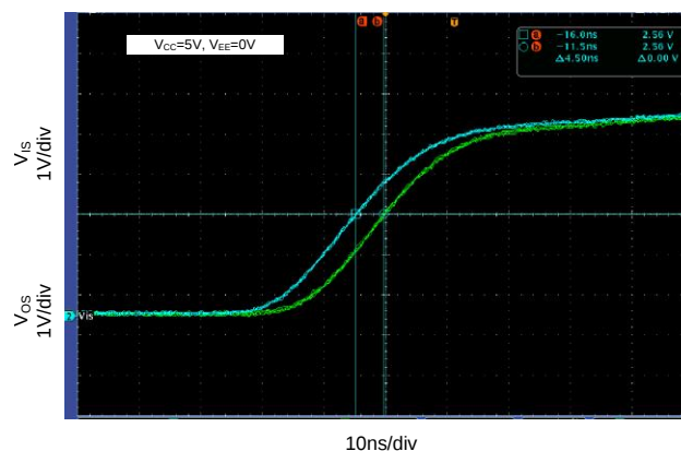
Figure 16. Propagation Delay
