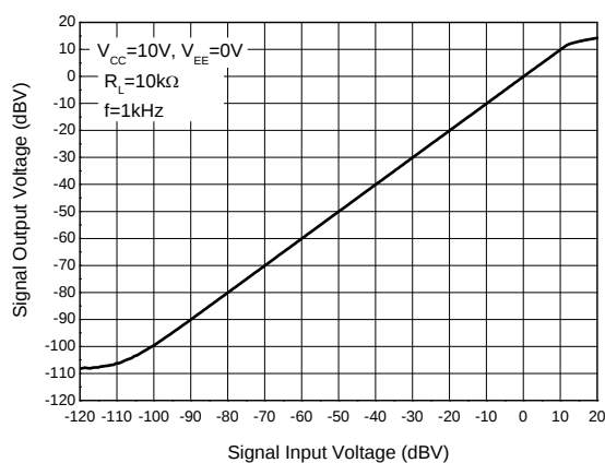
Figure 15. Linear Range
