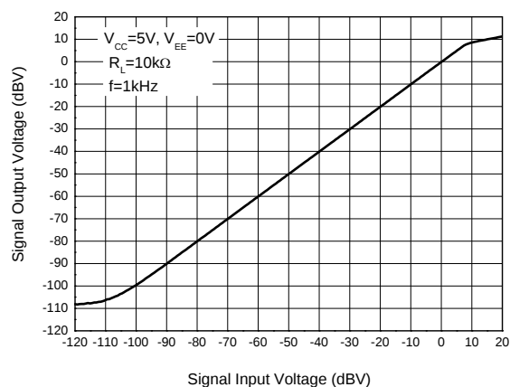
Figure 14. Linear Range
