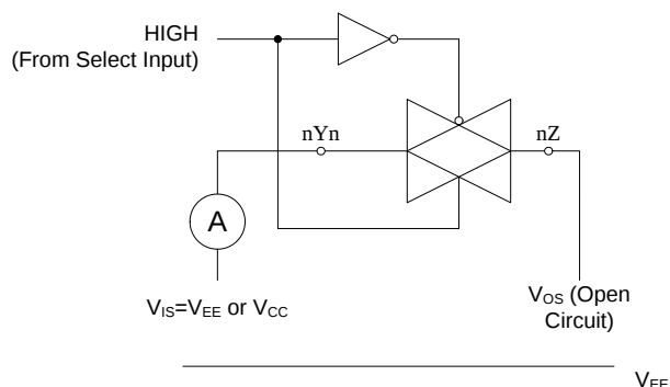
Figure 2. Test Circuit for Measuring ON-state Current
