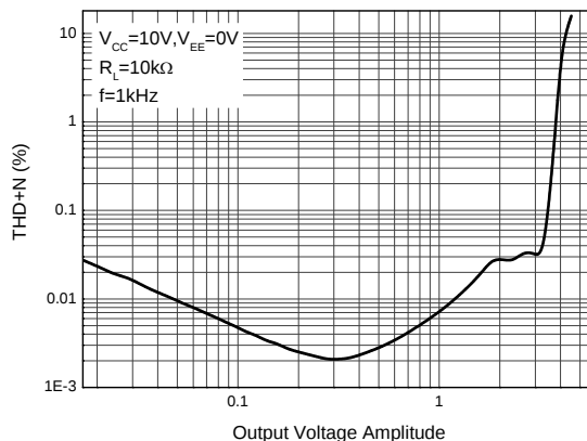
Figure 12. THD+N vs. Output Voltage Amplitude
