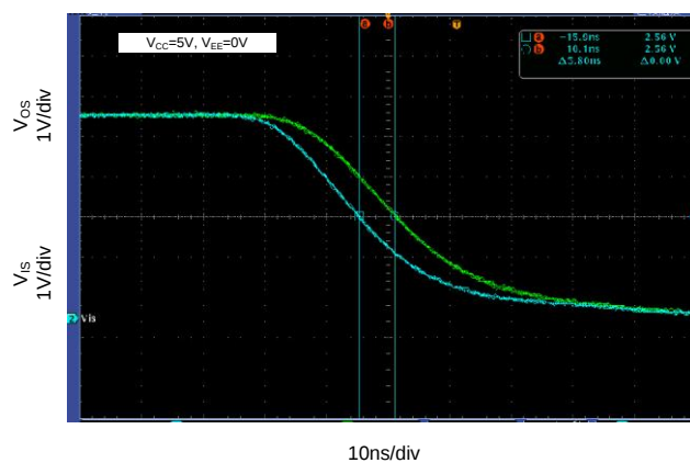
Figure 17. Propagation Delay
