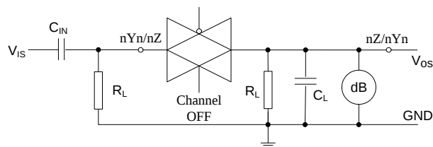
(b) Channel OFF Condition
