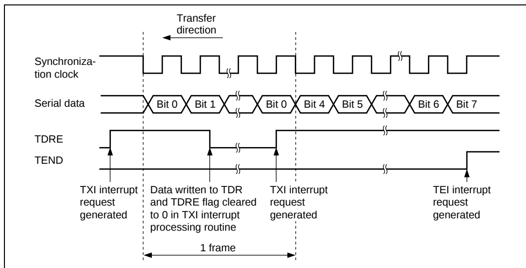
Figure 12.16 Sample SCI Transmission Operation in Clocked Synchronous Mode
