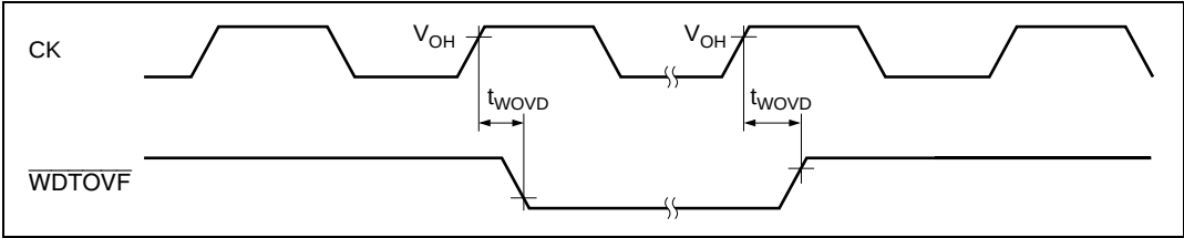
Figure 22.12 WDT Timing
