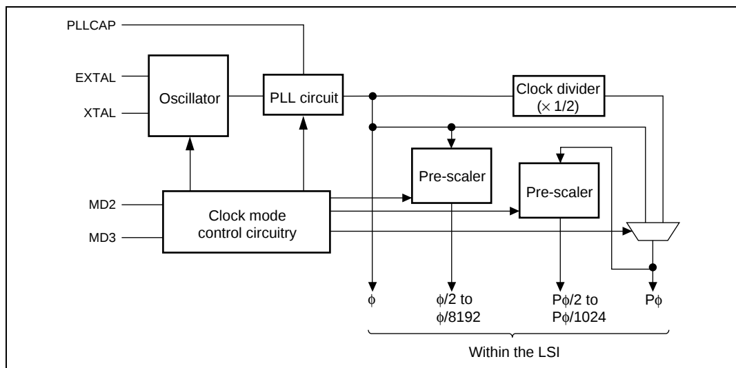
Figure 4.1 Block Diagram of the Clock Pulse Generator
