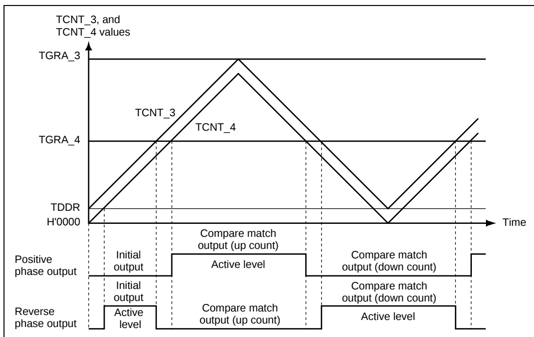
Figure 10.2 Complementary PWM Mode Output Level Example
