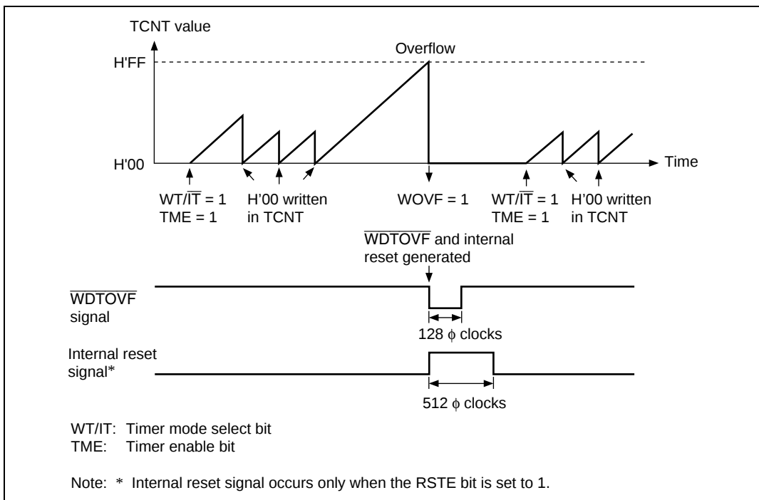
Figure 11.2 Operation in Watchdog Timer Mode
