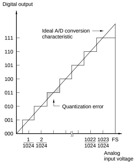
Figure 13.4 Definitions of A/D Conversion Accuracy
