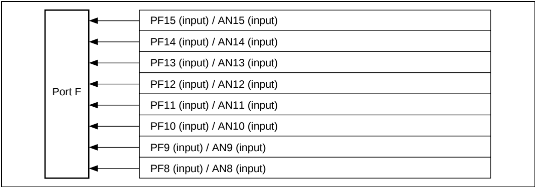
Figure 17.4 Port F
