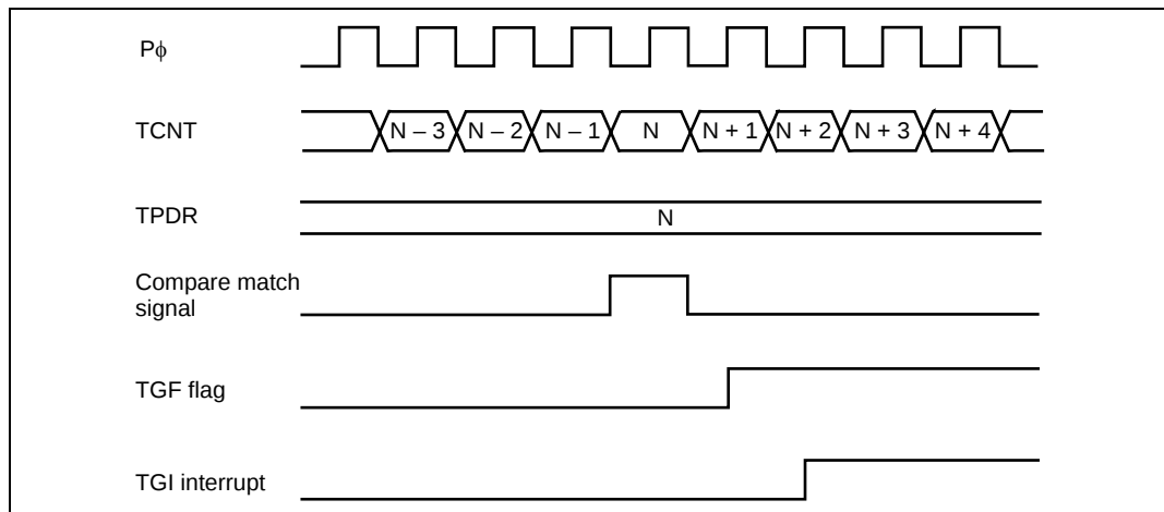
Figure 15.12 TGI Interrupt Timing
