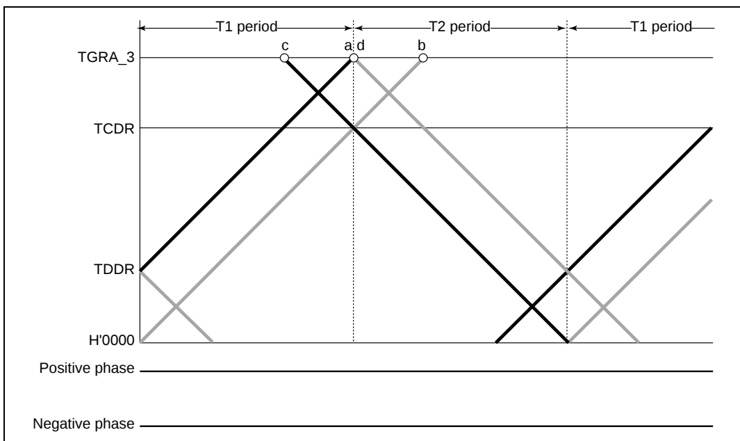
Figure 10.47 Example of Complementary PWM Mode 0% and 100% Waveform Output (5)
