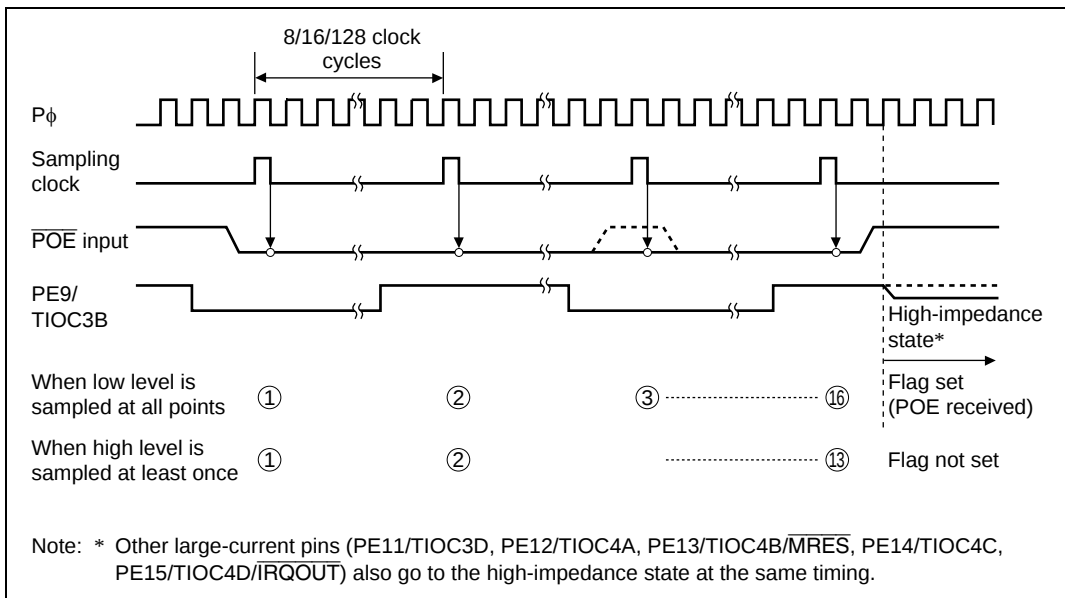
Figure 10.115 Low-Level Detection Operation
