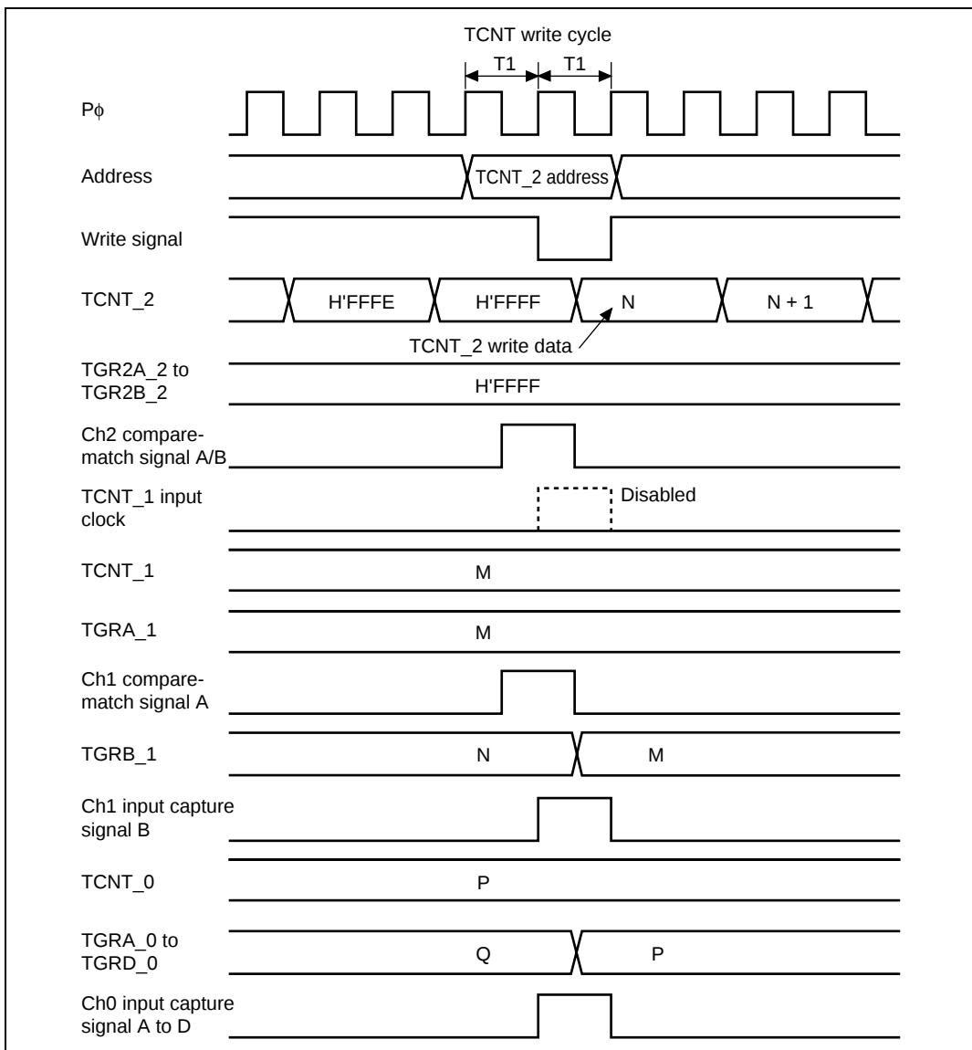
Figure 10.79 TCNT_2 Write and Overflow/Underflow Contention with Cascade Connection
