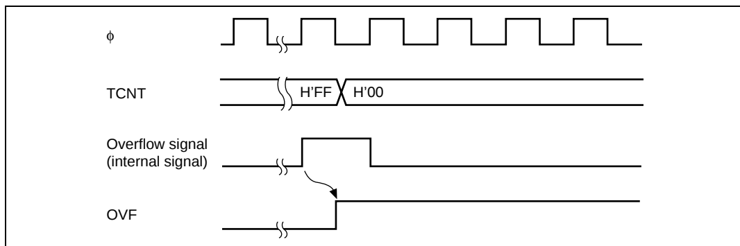
Figure 11.4 Timing of Setting OVF
