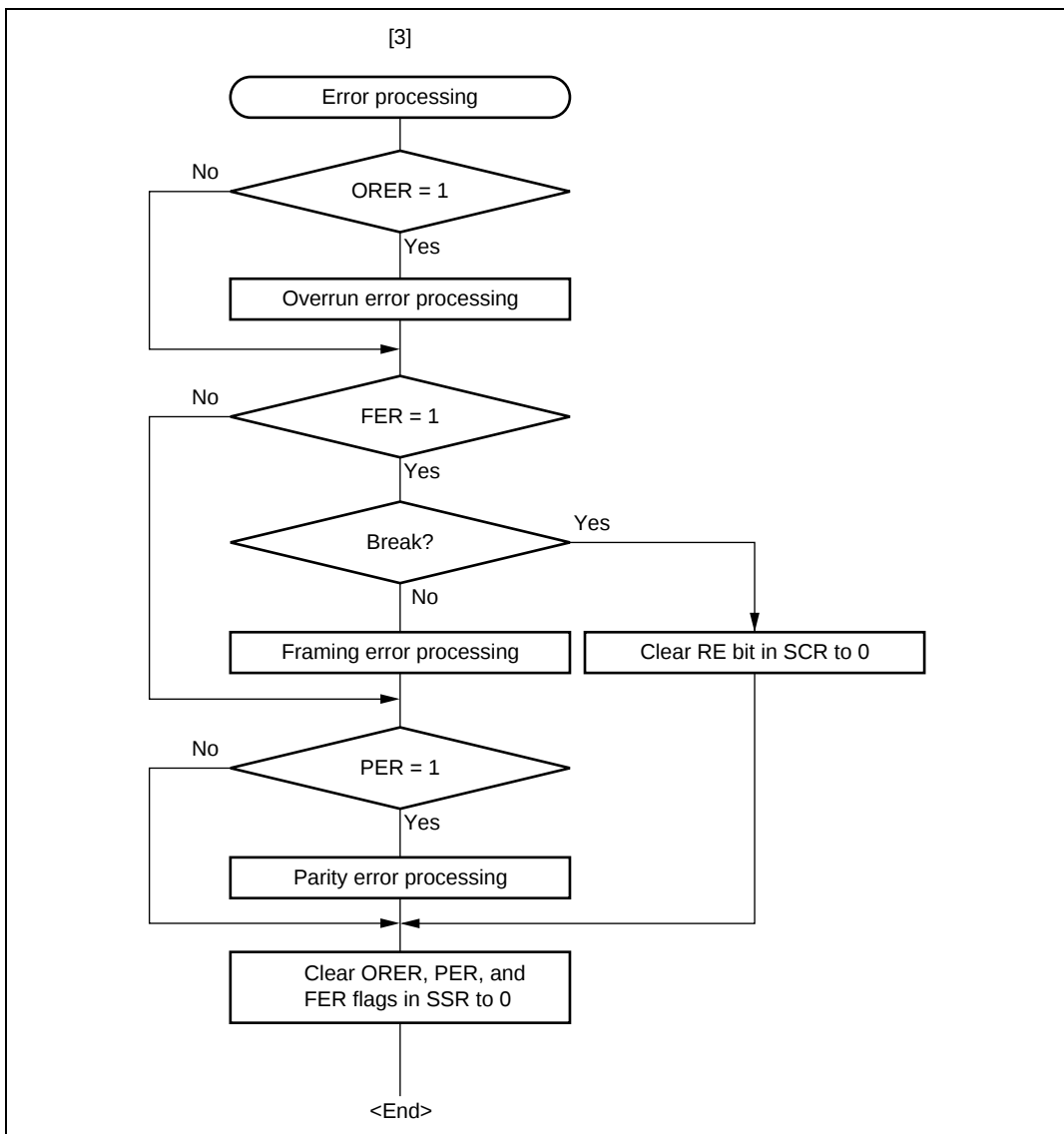
Figure 12.9 Sample Serial Reception Data Flowchart (2)
