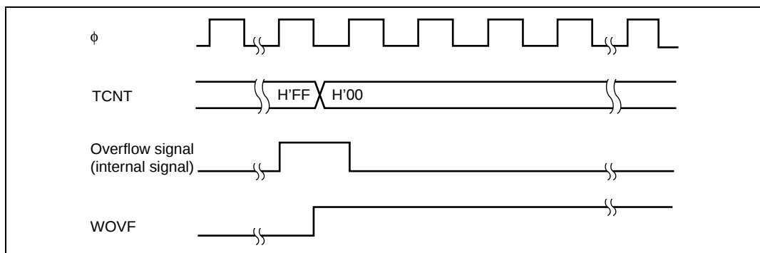
Figure 11.5 Timing of Setting WOVSF
