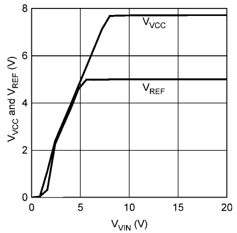
V_{VCC} and V_{REF} vs V_{VIN}
