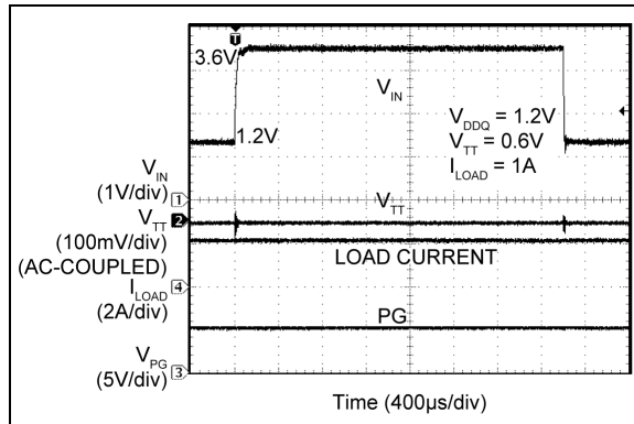
FIGURE 2-37: Line Transient.
