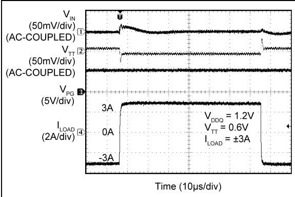
FIGURE 2-36: Load Transient (±3A).
