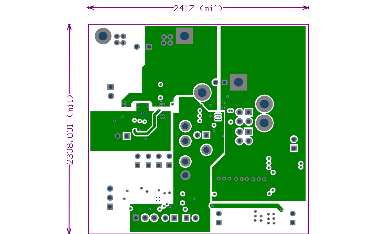
FIGURE 7-7: Copper Layer 3.
