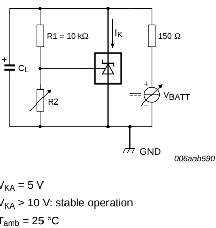
Fig 31. Test circuit (2) to Figure 29
