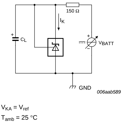
Fig 30. Test circuit (1) to Figure 29
