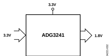
Figure 32. 3.3 V to 1.8 V Voltage Translation, \overline{SEL} = 0 V
