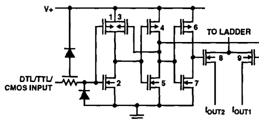
FIGURE 1. CMOS SWITCH
