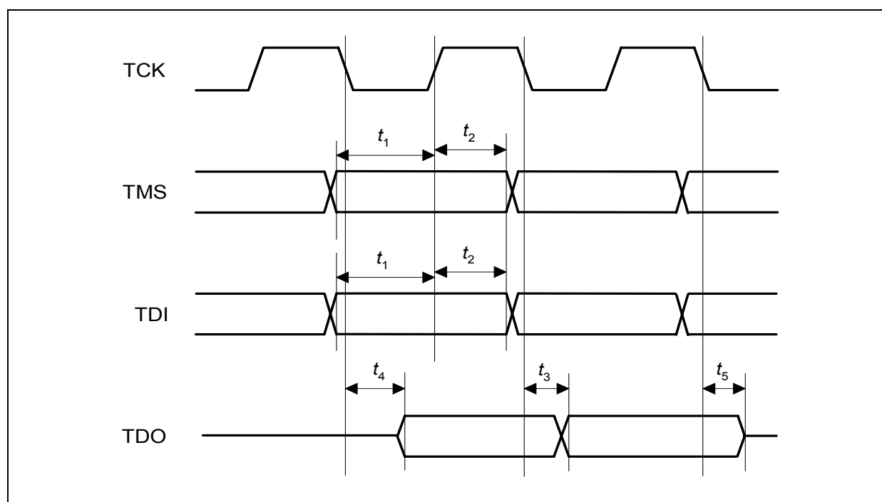
Figure 4-7 JTAG Timing
