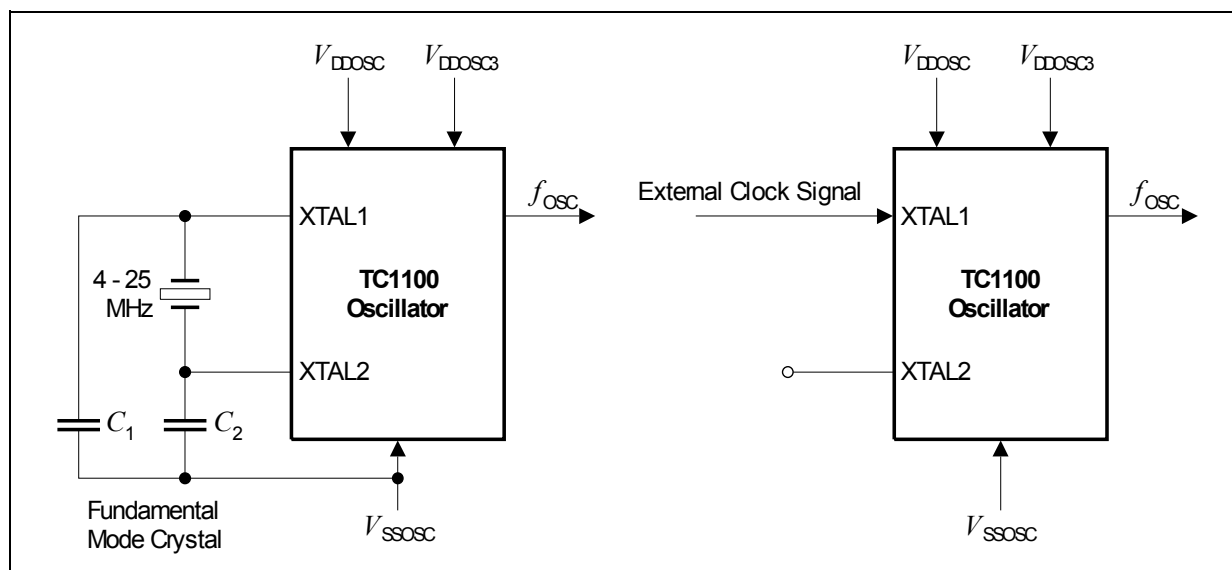
Figure 3-14 Oscillator Circuitries
