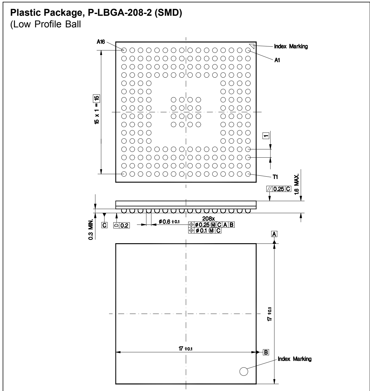
Figure 5-1 P-LBGA-208-2 Package
