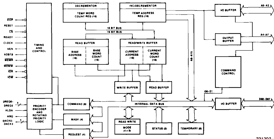
Figure 1. Block Diagram
