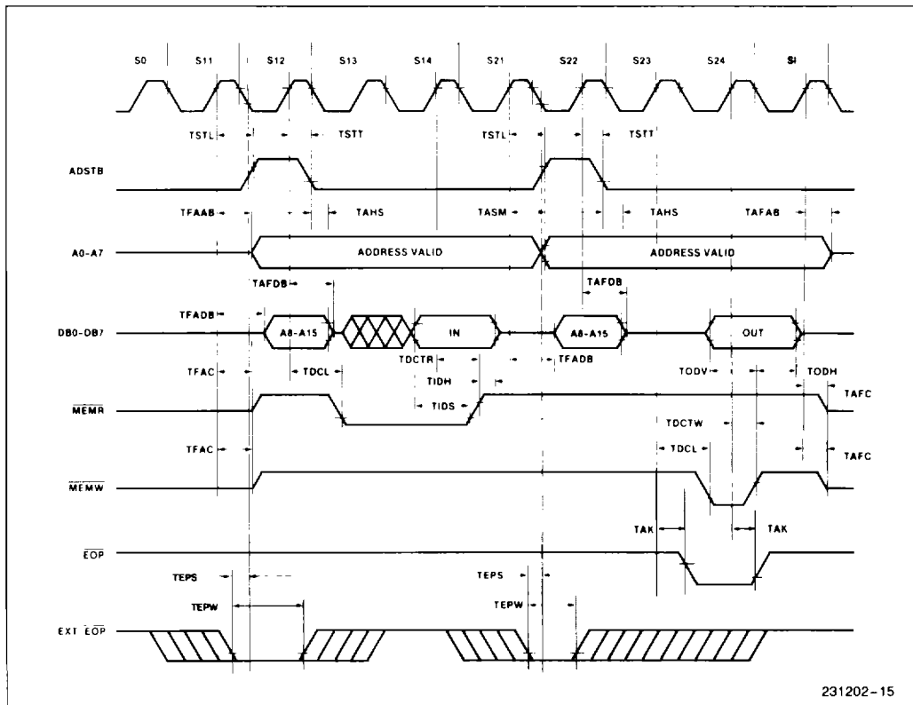
Figure 12. Memory-to-Memory Transfer
