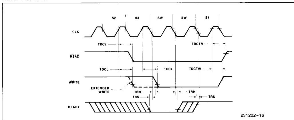
Figure 13. Ready
