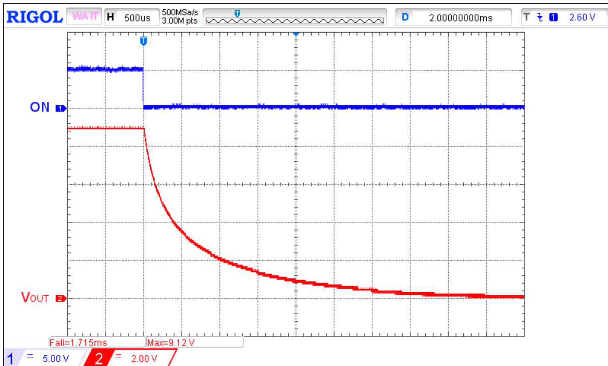
Figure 13. Typical Turn OFF operation waveform for V_{IN} = 9\text{ V} , C_{SLEW} = 10\text{ nF} , C_{LOAD} = 10\text{ μF} , R_{LOAD} = 100\text{ Ω}
