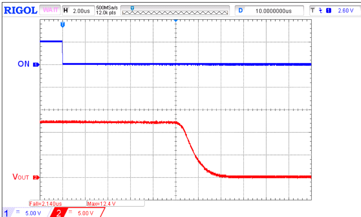
Figure 14. Typical Turn OFF operation waveform for V_{IN} = 12\text{ V} , C_{SLEW} = 10\text{ nF} , no C_{LOAD} , R_{LOAD} = 100\text{ Ω}
