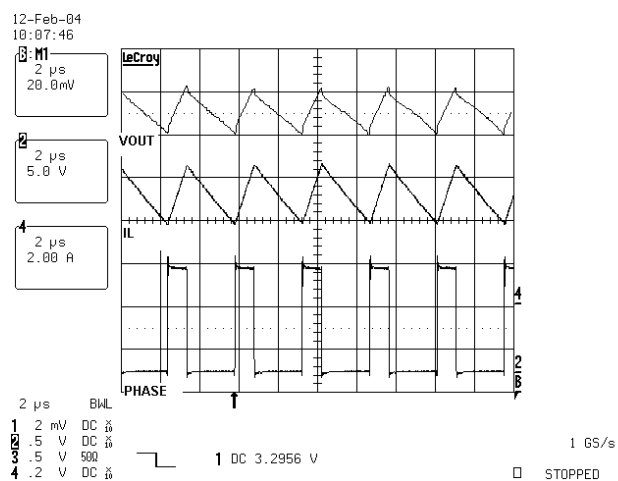
FIGURE 5. PWM WAVEFORMS
