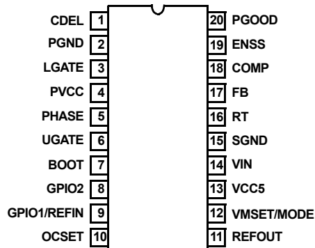
ISL6420 (20 LD QSOP) TOP VIEW
