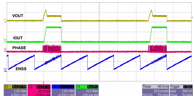
FIGURE 9. TYPICAL OVER-CURRENT HICCUP MODE
