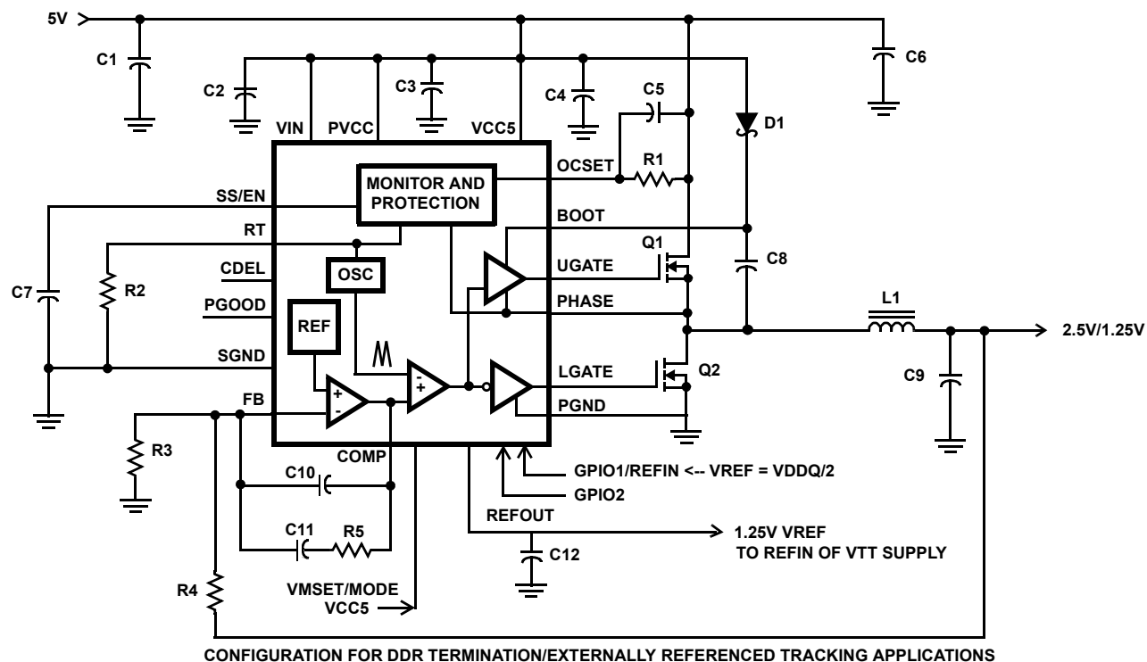
Typical 5V Input DC/DC Application Schematic
