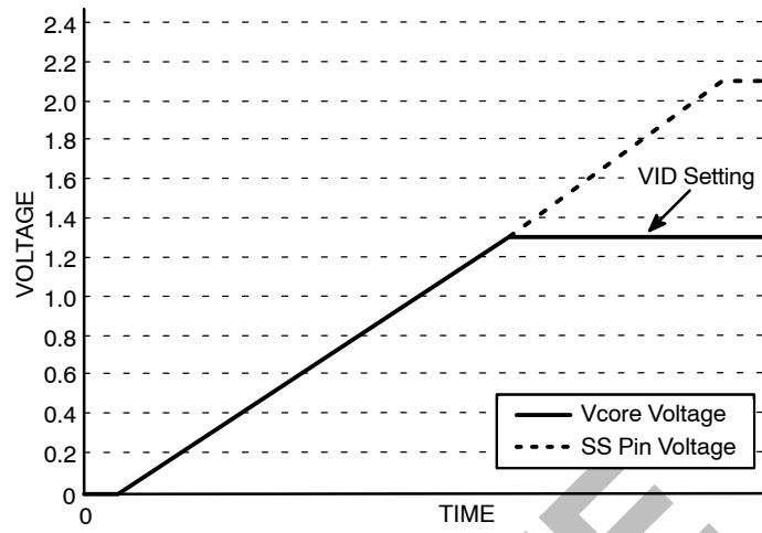
Figure 9. Typical VR10 Soft-Start Sequence to V_{core} = 1.3\text{ V}
