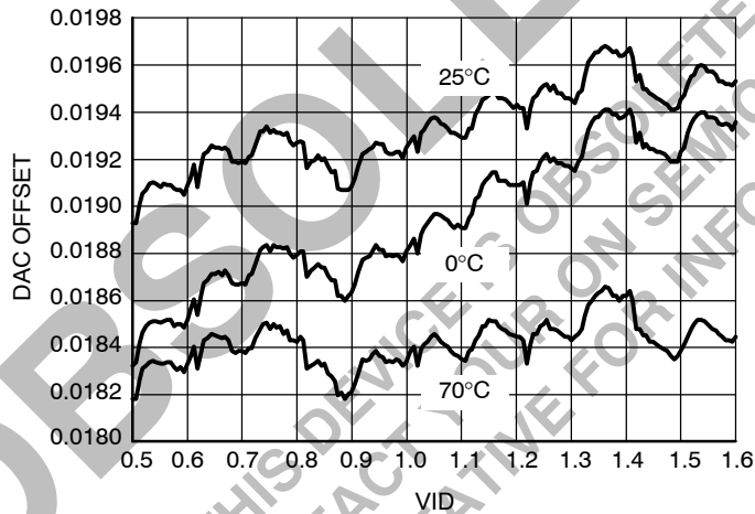
Figure 8. Typical DAC Voltage Offset vs. Temperature
