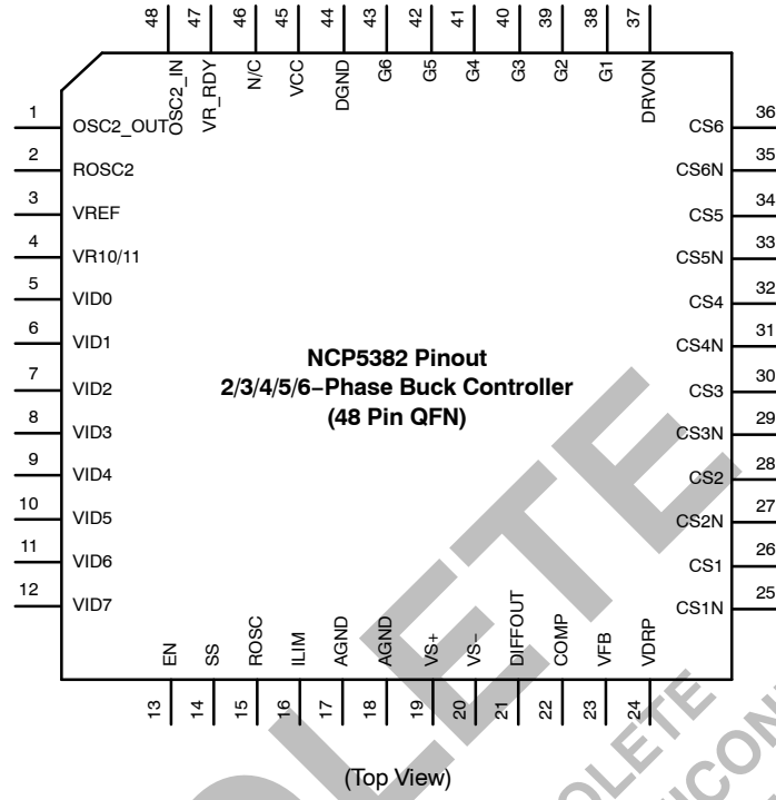
Figure 1. Pinout
