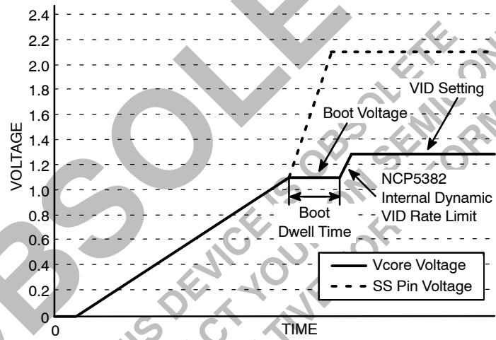
Figure 10. Typical VR11 Soft-Start Sequence to V_{core} = 1.3\text{ V}
