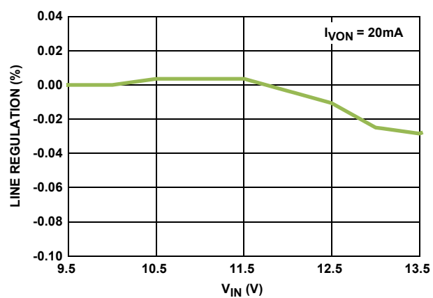
FIGURE 18. V_{ON} LINE REGULATION
