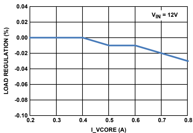
FIGURE 14. Vcore BUCK LOAD REGULATION
