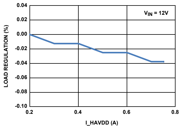
FIGURE 6. HAVDDBUCK REGULATION
