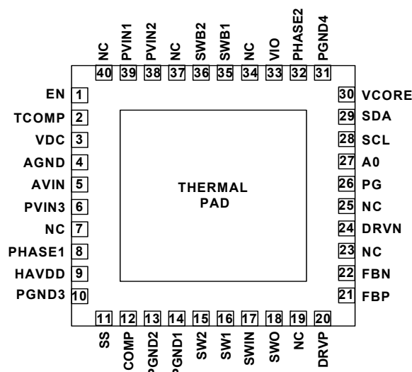
ISL98604 (40 LD 5x5 TQFN) TOP VIEW
