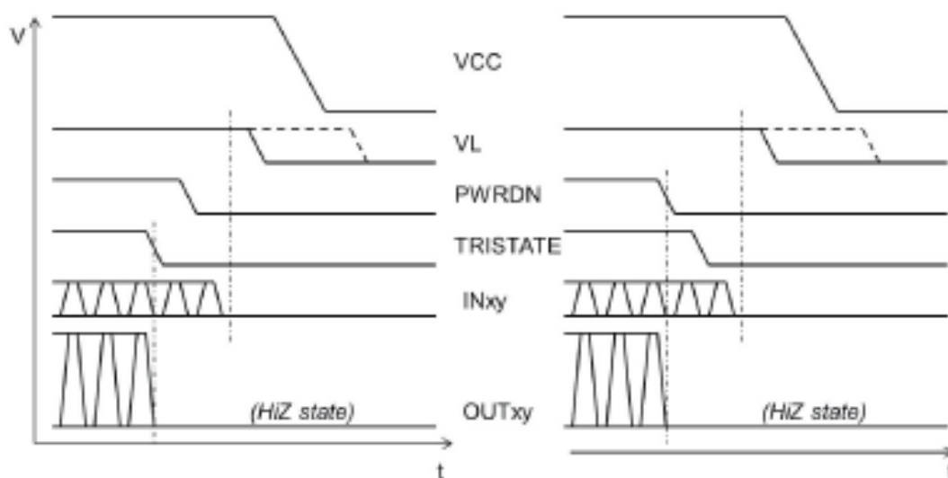
Figure 5. Power-OFF sequence
