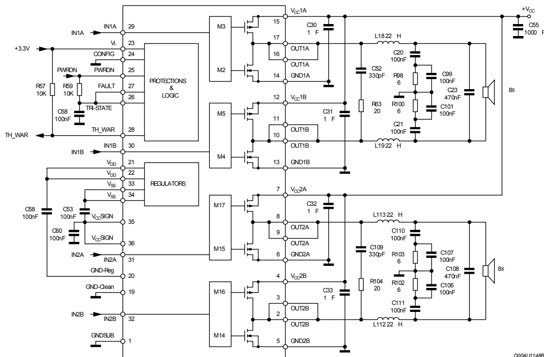
Figure 8. Typical audio application circuit (dual BTL)
