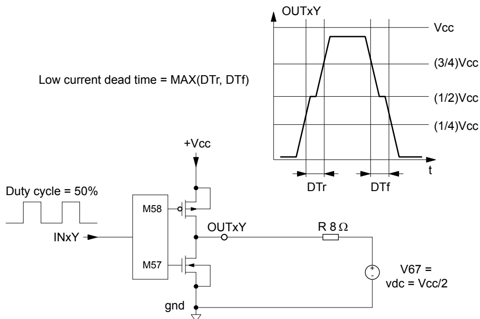
Figure 2. Test circuit
