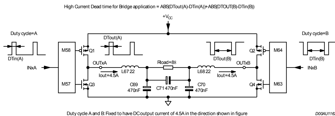
Figure 3. Current dead-time test circuit
