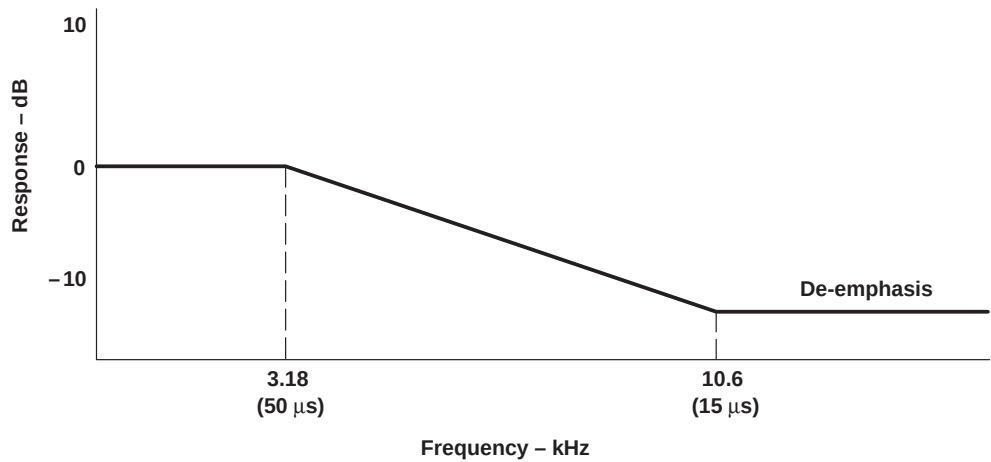
Figure 4. De-emphasis Characteristics
