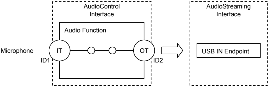
Figure 19. AK5373 Topology
