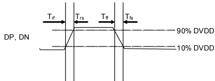
Figure 4. Rise/Fall Time
