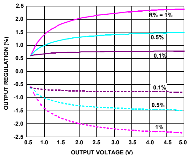
FIGURE 33. OUTPUT REGULATION WITH DIFFERENT RESISTOR TOLERANCE FOR \text{Ref}\% = \pm 0.6\%
