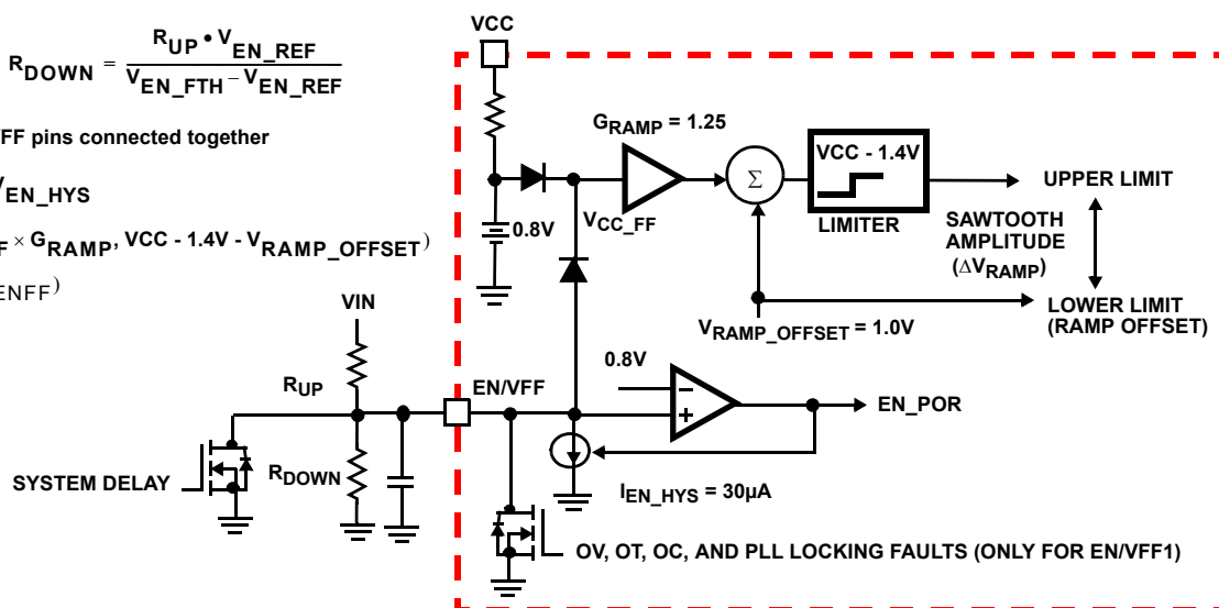
FIGURE 12. SIMPLIFIED ENABLE AND VOLTAGE FEED-FORWARD CIRCUIT
