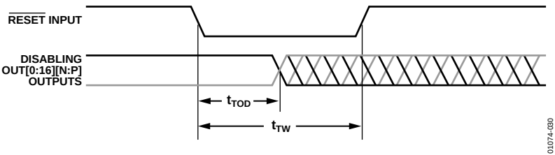
Figure 30, Asynchronous Reset
