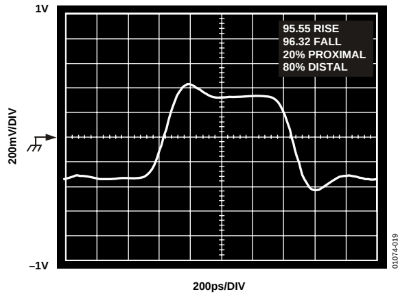
Figure 19. Rise/Fall Times, V_{EE} = -3.3 V
