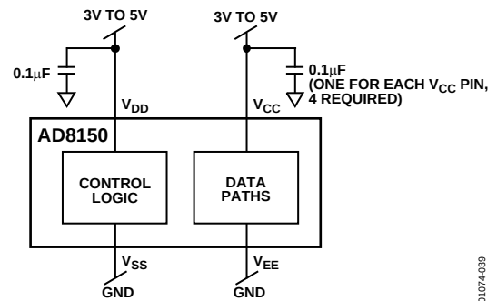
Figure 39. Power Supplies and Bypassing for PECL Operation
