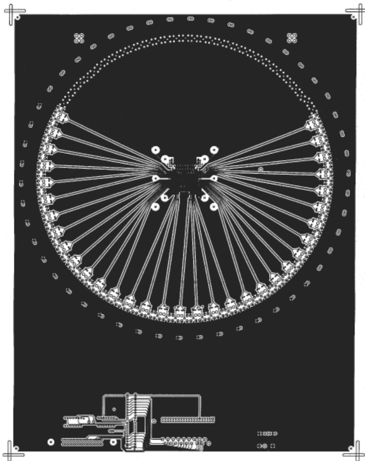
Figure 44. Circuit Side
