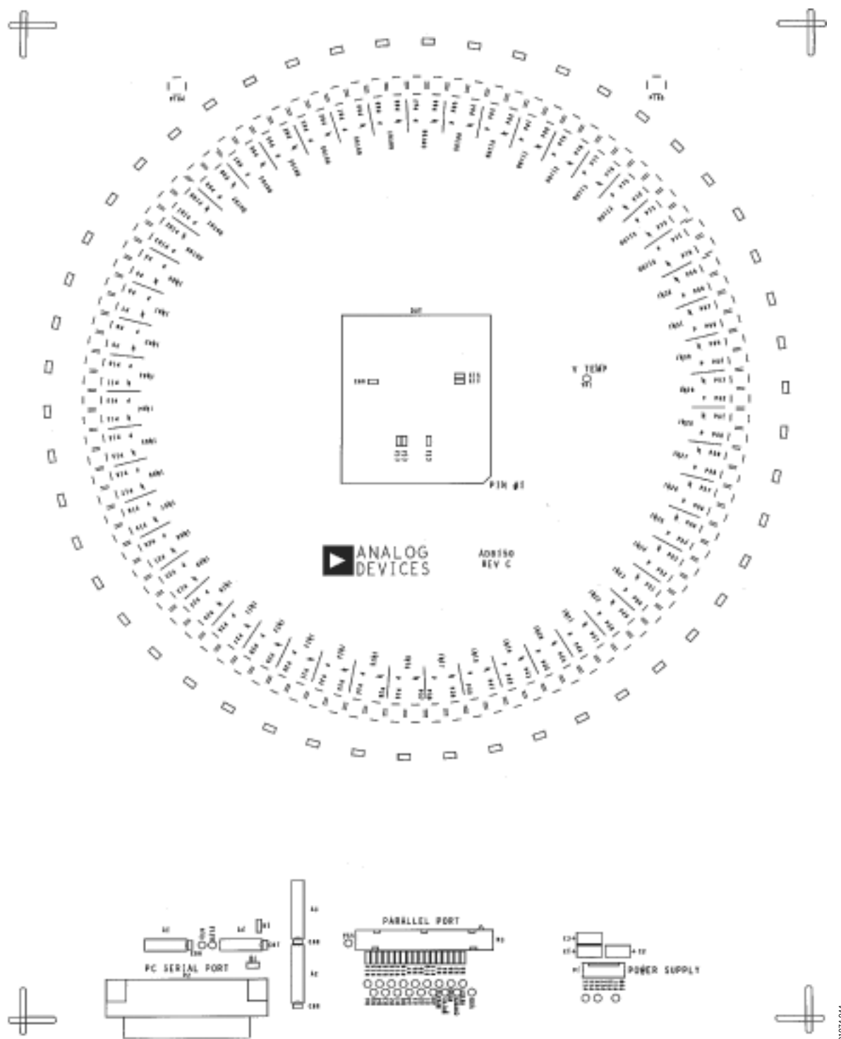
Figure 45. Silkscreen Top
