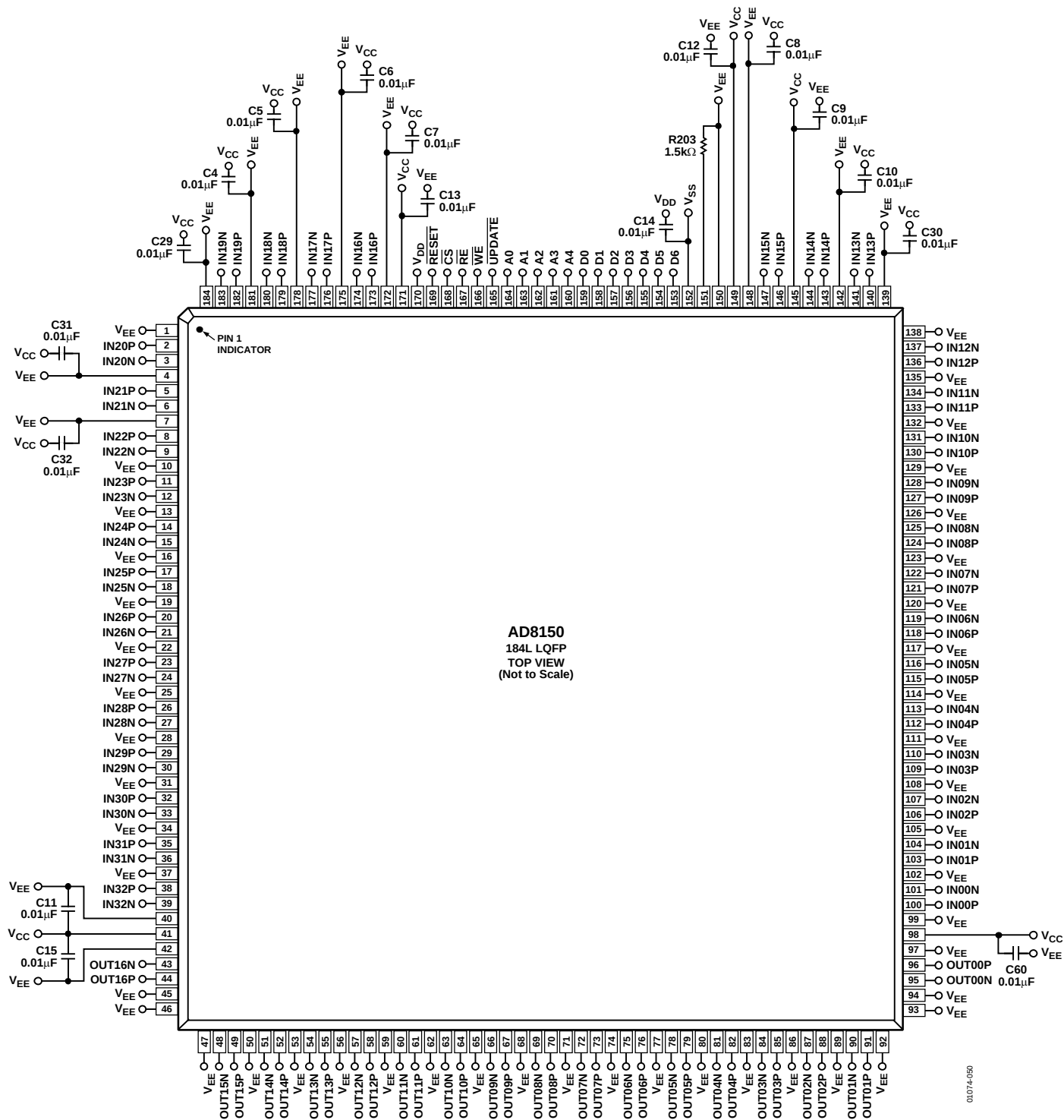
Figure 40. Bypassing Schematic
