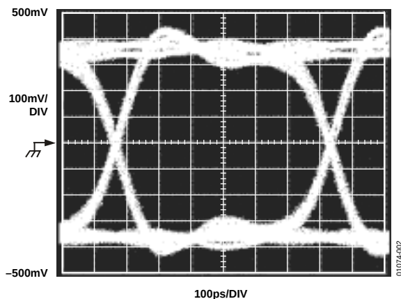
Figure 2. Output Eye Pattern, 1.5 Gbps
