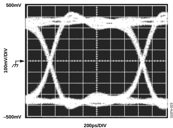
Figure 23. Eye Pattern, V_{EE} = -3.3\text{ V} , 1.5 Gbps PRBS 23
