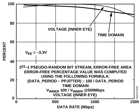
Figure 13. AC Performance
