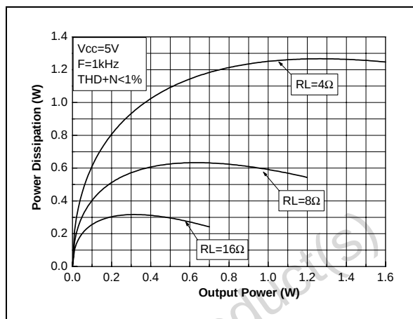
Figure 53: Power dissipation vs. output power: speaker output
