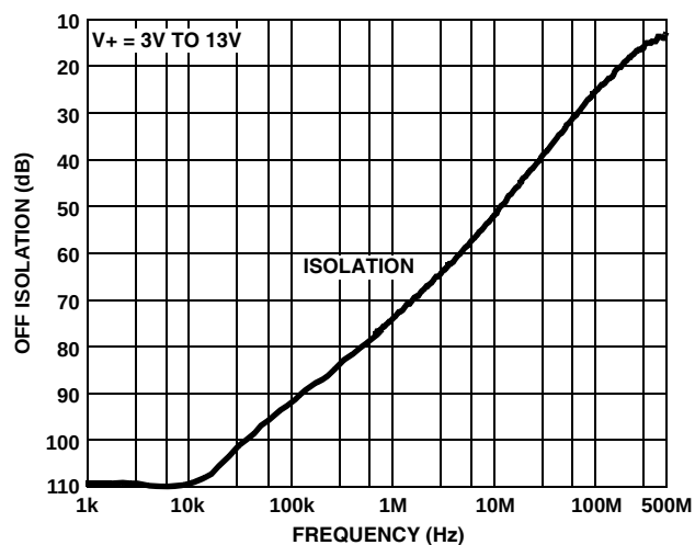
FIGURE 17. OFF ISOLATION
