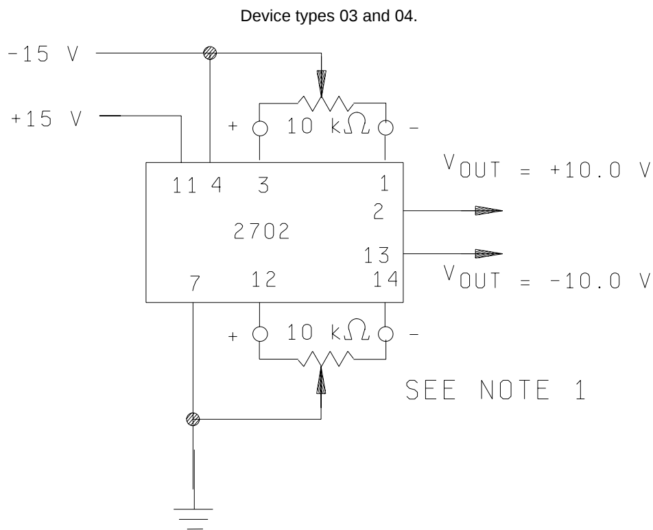
FIGURE 3. Trim circuit(s).
