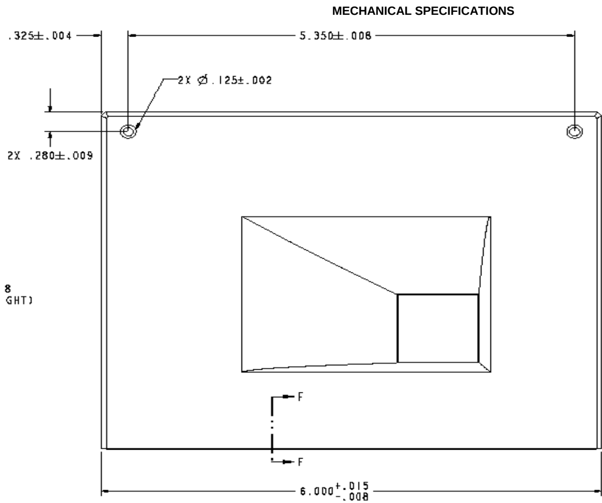
Figure 24. S.E.C. Cartridge Retention Enabling Details (Notes follow)
