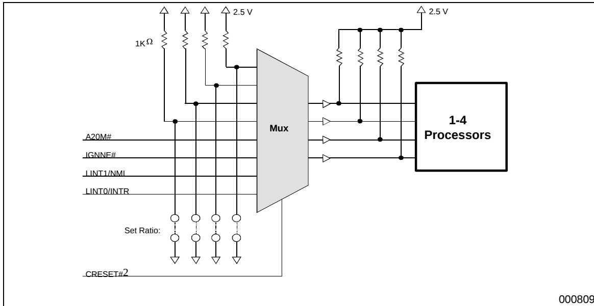
Figure 2. Logical1 Schematic for Clock Ratio Pin Sharing
