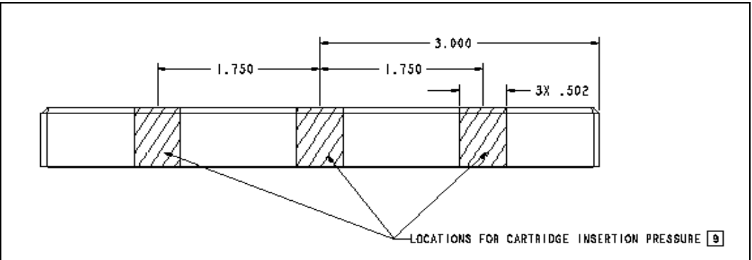
Figure 27. Top View of Cartridge Insertion Pressure Points
