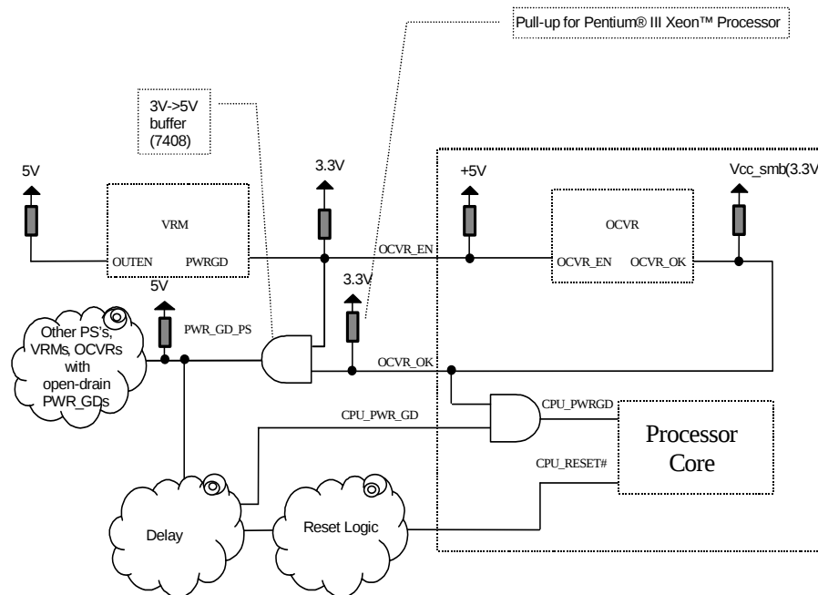
Figure 42. PWRGD Implementation
