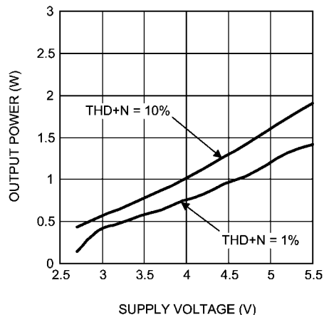
OUTPUT POWER vs SUPPLY VOLTAGE R_L = 8\Omega , Stereo Mode, ADC Input
