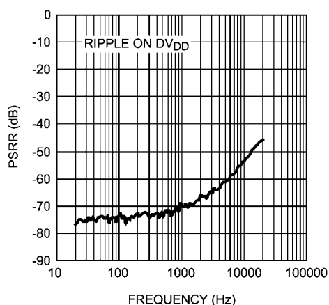
PSRR vs FREQUENCY PV_{DD} = 5V , V_{RIPPLE} = 200mV_{P-P} , R_L = 8\Omega , I^2S input = -120dBFS
