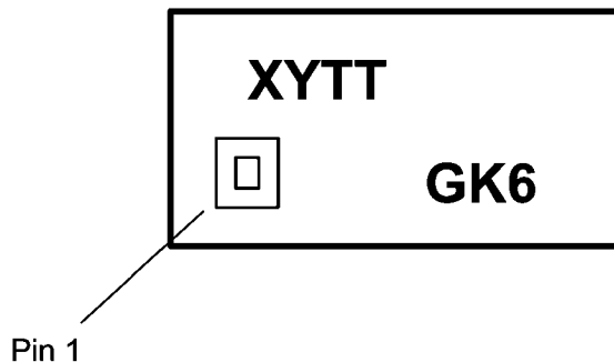
Top View XY = Date code TT = Die traceability G = Boomer Family K6 = LM48903TL
