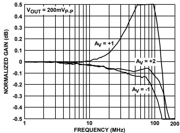
FIGURE 19. GAIN FLATNESS
