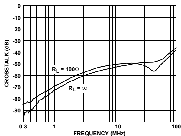
FIGURE 21. ALL HOSTILE CROSSTALK
