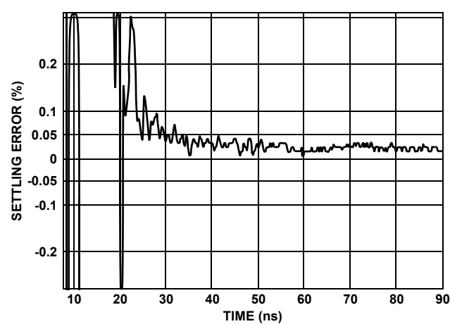
FIGURE 33. SETTLING RESPONSE
