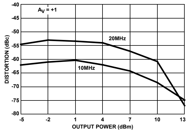
FIGURE 25. 3rd HARMONIC DISTORTION vs P_{\text{OUT}}
