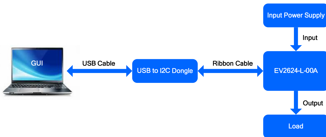
EVKT-2624 Evaluation Kit Set-Up
