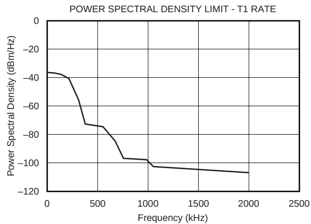
CURVE 1. Upper Bound of Power Spectral Density Measured at Output of HDSL Transformer.
