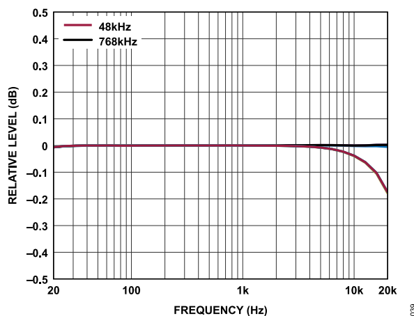
Figure 39. Relative Level vs. Frequency, Headphone Mode (16 \Omega ) or Line Output Mode (10 k \Omega ), f_s = 48 kHz and 768 kHz, Signal Path = AINx to DAC, ADC0 and ADC1 Differential Mode, ADC2 Single-Ended Mode
