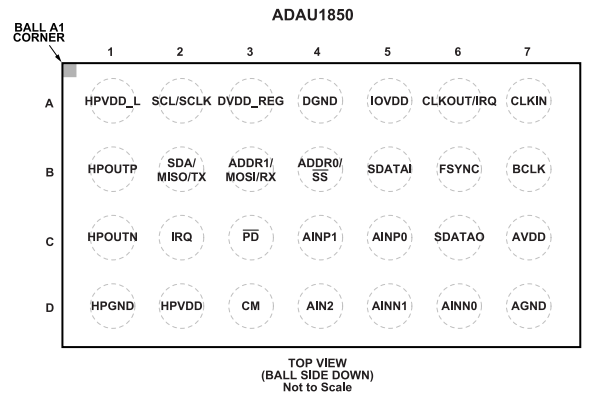
Figure 6. Pin Configuration (Top View)
