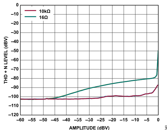
Figure 40. THD + N Level vs. Amplitude, f_s = 48 kHz to 768 kHz, Signal Path = AINx to Headphone Mode (16 \Omega ) or Line Output Mode (10 k \Omega ), ADC0 and ADC1 Differential Mode
