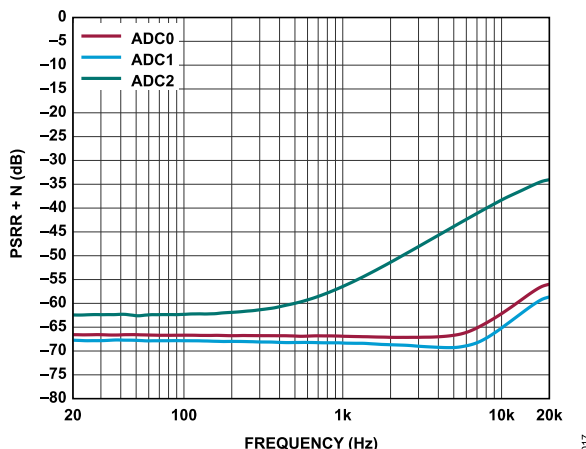
Figure 17. PSRR + N, Signal Path = AINx to SDATAO, f_s = 48 kHz, 100 mV p-p Ripple Input on AVDD, PGA = 10 dB, ADC0 and ADC1 Differential Mode, ADC2 Single-Ended Mode
