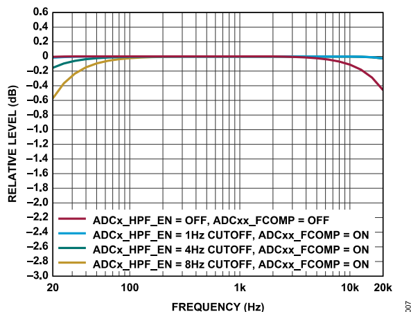
Figure 7. Frequency Response, f_s = 48 kHz, -20 dBV Input, Signal Path = AINx to SDATAO, No PGA, ADC0 and ADC1 Differential Mode, ADC2 Single-Ended Mode
