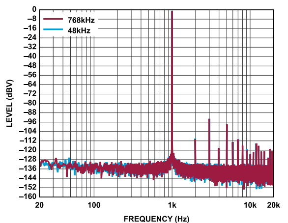
Figure 42. FFT, -1 dBV, Line Output Mode, Load = 10 k \Omega , f_s = 48 kHz to 768 kHz, Signal Path = AINx to DAC, ADC0 and ADC1 Differential Mode
