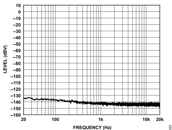
Figure 20. FFT, No Signal, f_s = 48 kHz, Signal Path = SDATAI to Headphone Output, Line Output Mode, Load = 10\ k\Omega
