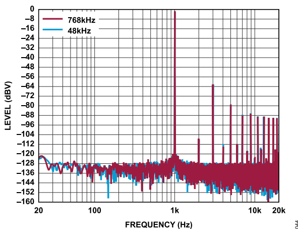
Figure 44. FFT, -1 dBV, Headphone Mode, Load = 16 \Omega , f_s = 48 kHz to 768 kHz, Signal Path = AINx to DAC, ADC0 and ADC1 Differential Mode
