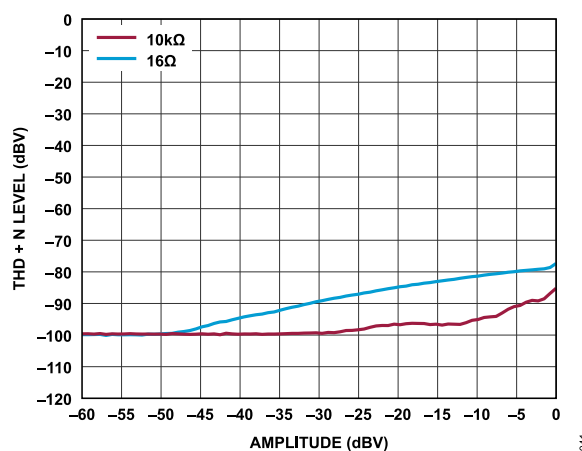
Figure 41. THD + N Level vs. Amplitude, f_s = 48 kHz to 768 kHz, Signal Path = AINx to Headphone Mode (16 \Omega ) or Line Output Mode (10 k \Omega ), ADC2 Single-Ended Mode
