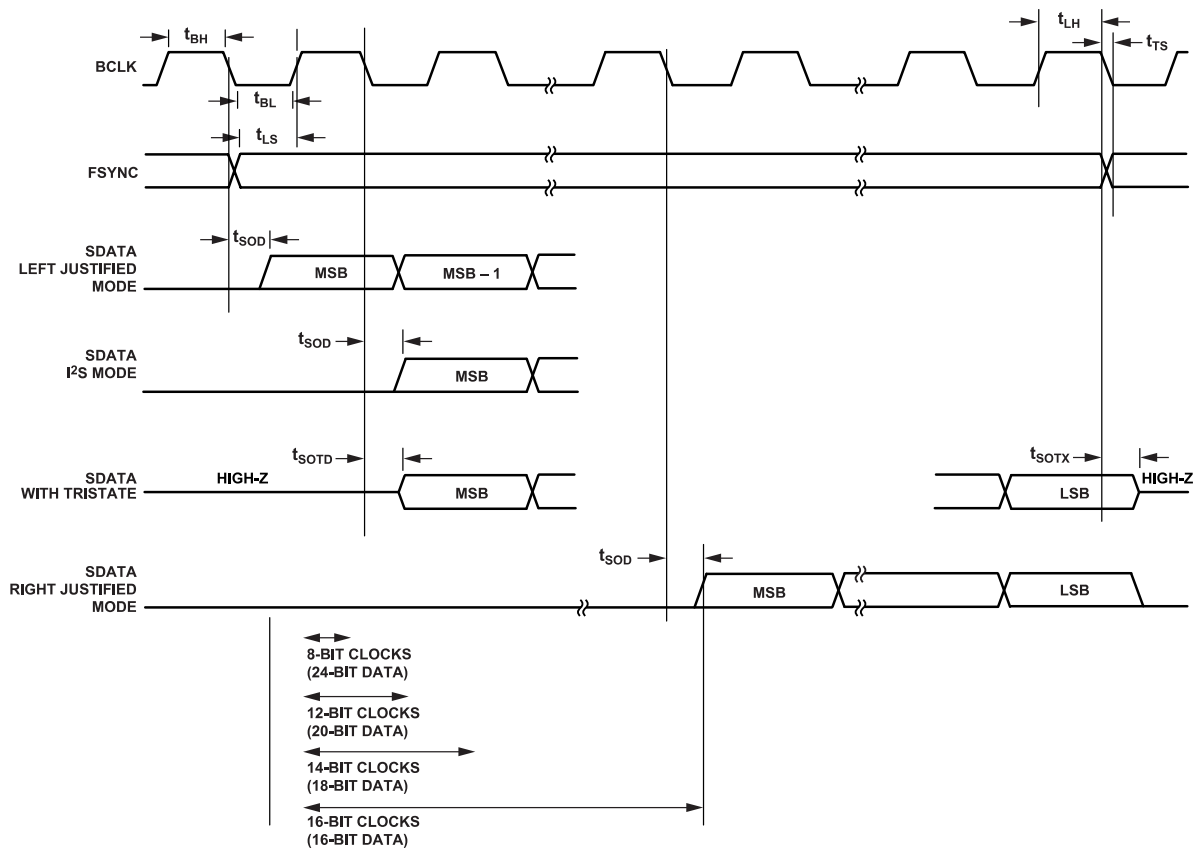
Figure 3. Serial Output Port Timing Diagram
