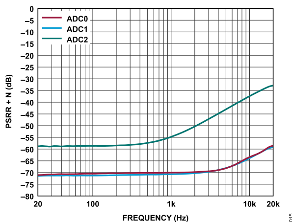
Figure 15. PSRR + N, Signal Path = AINx to SDATAO, f_s = 48 kHz, 100 mV p-p Ripple Input on AVDD, No PGA, ADC0 and 1 Differential Mode, ADC2 Single-Ended Mode
