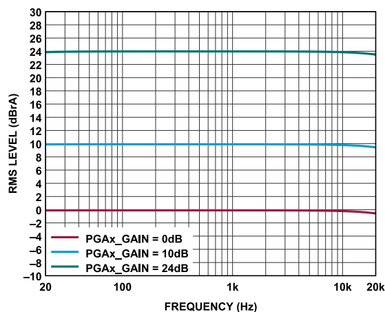
Figure 8. Frequency Response, f_s = 48 kHz, Signal Path = AINx to SDATAO, Output Relative to PGA Gain Settings (0 dB, 10 dB, 24 dB)
