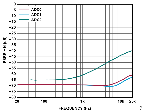
Figure 16. PSRR + N, Signal Path = AINx to SDATAO, f_s = 48 kHz, 100 mV p-p Ripple Input on AVDD, PGA = 0 dB, ADC0 and ADC1 Differential Mode, ADC2 Single-Ended Mode
