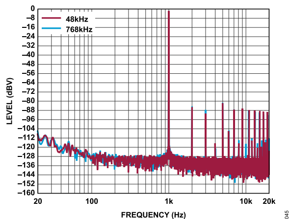
Figure 45. FFT, -1 dBV, Headphone Mode, Load = 16 \Omega , f_s = 48 kHz to 768 kHz, Signal Path = AINx to DAC, ADC2 Single-Ended Mode
