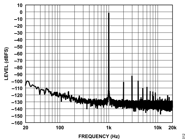
Figure 12. FFT, -7 dBV Input, -1 dBFS Output, f_s = 48 kHz, Signal Path = AINx to SDATAO, No PGA, ADC2 Single-Ended Mode
