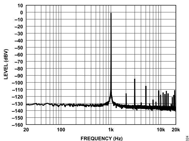
Figure 24. FFT, -1 dBFS, f_s = 48 kHz, Signal Path = SDATAI to Headphone Output, Line Output Mode, Load = 10\ k\Omega
