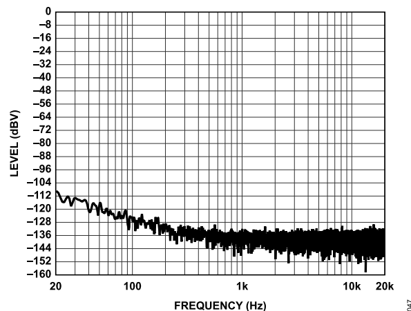
Figure 47. FFT, No Signal, f_s = 48 kHz to 768 kHz, Signal Path = AINx to DAC Headphone Mode (16 \Omega ) or Line Output Mode (10 k \Omega ), ADC2 Single-Ended Mode
