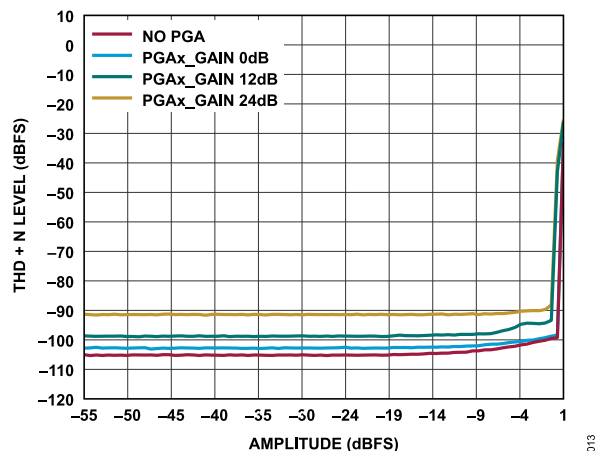
Figure 13. THD + N Level vs. Amplitude, f_s = 48 kHz, Signal Path = AINx to SDATAO, No PGA and PGA Gain Settings (0 dB, 12 dB, 24 dB), ADC0 and ADC1 Differential Mode
