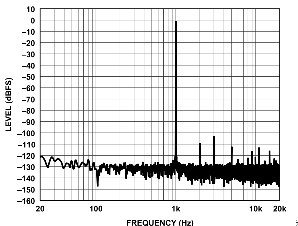
Figure 11. FFT, -7 dBV Input, -1 dBFS Output, f_s = 48 kHz, Signal Path = AINx to SDATAO, No PGA, ADC0 and ADC1 Differential Mode
