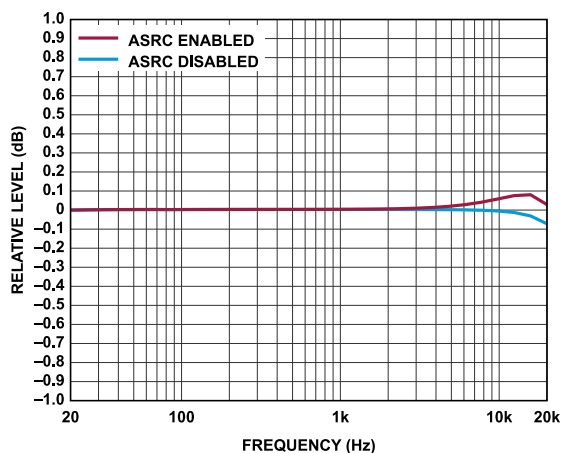
Figure 32. Relative Level vs. Frequency, f_s = 48 kHz Throughout Except FastDSP = 768 kHz, Signal Path = SDATAI to ASRCI to Equalizer to Interpolator to FastDSP to Decimator to ASRCO to SDATAO
