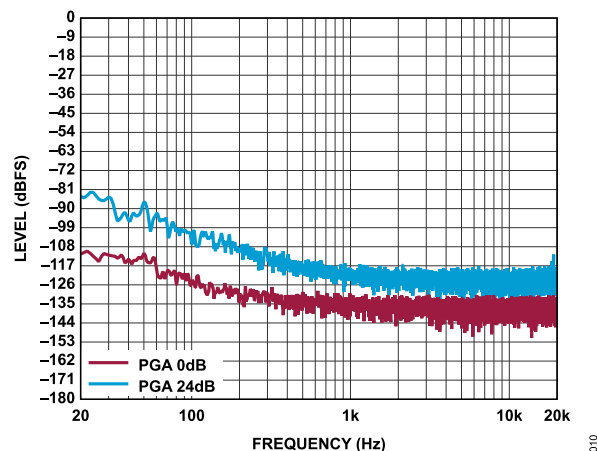
Figure 10. FFT, No Signal, f_s = 48 kHz, Signal Path = AINx to SDATAO, PGA = 0 dB and 24 dB (PGAx_GAIN), ADC2 Single-Ended Mode
