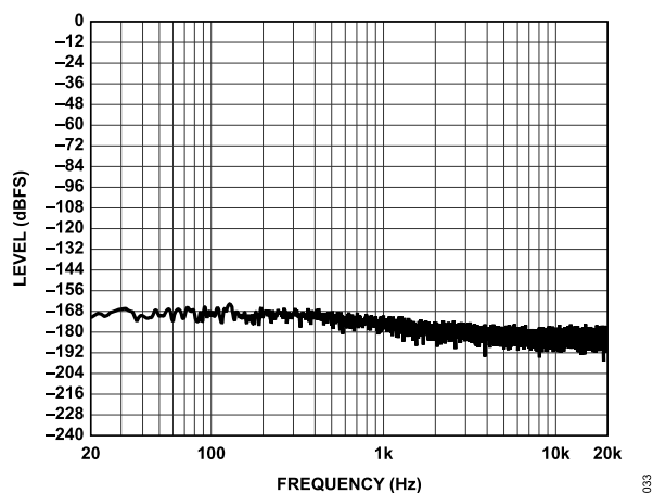
Figure 33. FFT, No Signal, f_s = 48 kHz Throughout Except FastDSP = 768 kHz, Signal Path = SDATAI to ASRCI to Equalizer to Interpolator to FastDSP to Decimator to ASRCO to SDATAO
