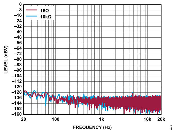
Figure 46. FFT, No Signal, f_s = 48 kHz to 768 kHz, Signal Path = AINx to DAC Headphone Mode (16 \Omega ) or Line Output Mode (10 k \Omega ), ADC0 and ADC1 Differential Mode
