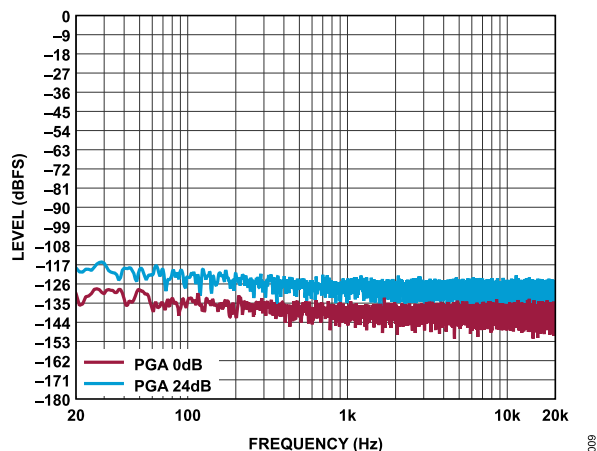
Figure 9. FFT, No Signal, f_s = 48 kHz, Signal Path = AINx to SDATAO, PGA = 0 dB and 24 dB (PGAx_GAIN), ADC0 and ADC1 Differential Mode
