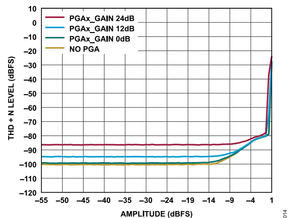
Figure 14. THD + N Level vs. Amplitude, f_s = 48 kHz, Signal Path = AINx to SDATAO, No PGA and PGA Gain Settings (0 dB, 12 dB, 24 dB), ADC2 Single-Ended Mode
