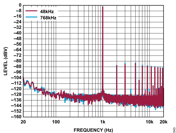
Figure 43. FFT, -1 dBV, Line Output Mode, Load = 10 k \Omega , f_s = 48 kHz to 768 kHz, Signal Path = AINx to DAC, ADC2 Single-Ended Mode
