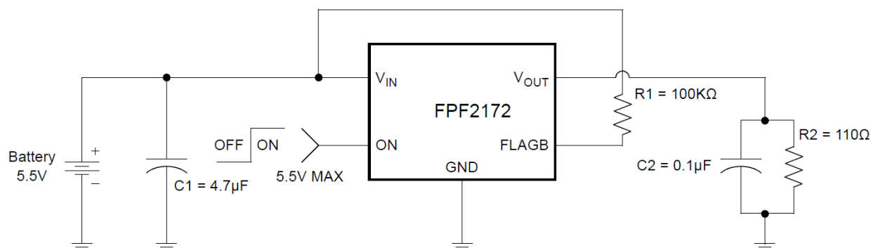
Figure 22. Typical Application
