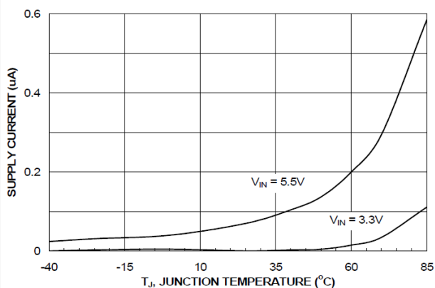
Figure 7. I_{SWITCH-OFF} Current vs. Temperature
