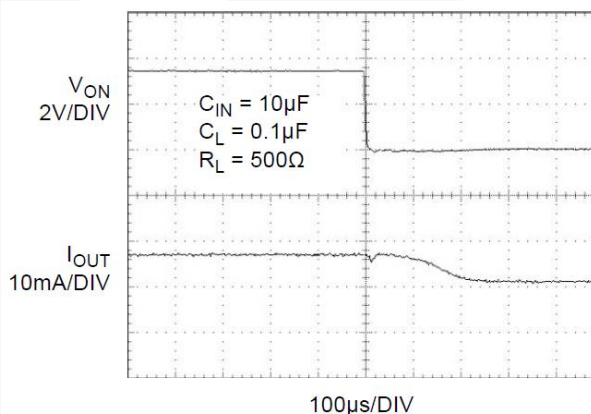
Figure 19. t_{OFF} Response
