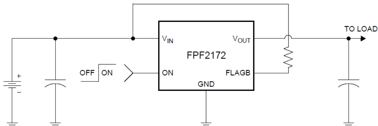
Figure 1. Typical Application
