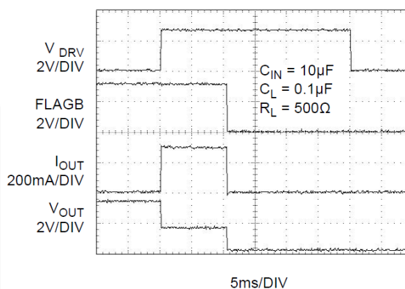
Figure 17. t_{BLANK} Response
