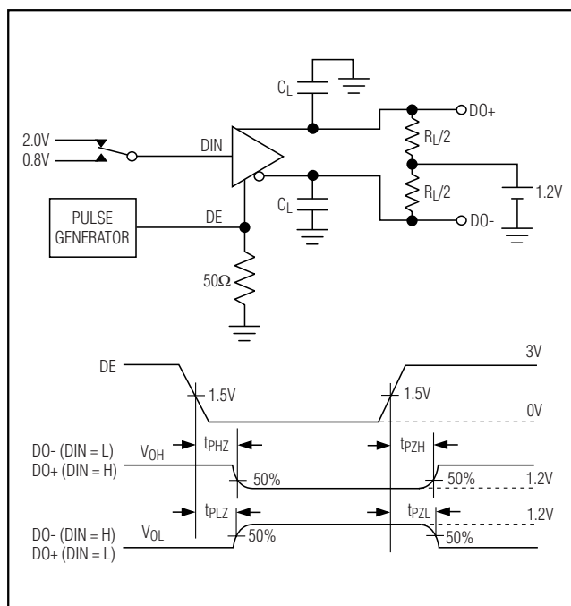
Figure 3. Driver High-Impedance Delay Test Circuit and Waveforms
