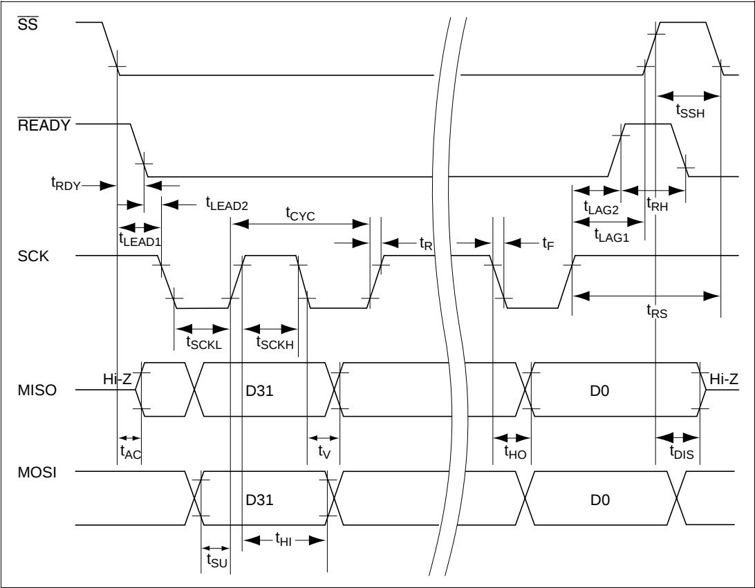
Figure 12-13 SPI Timing
