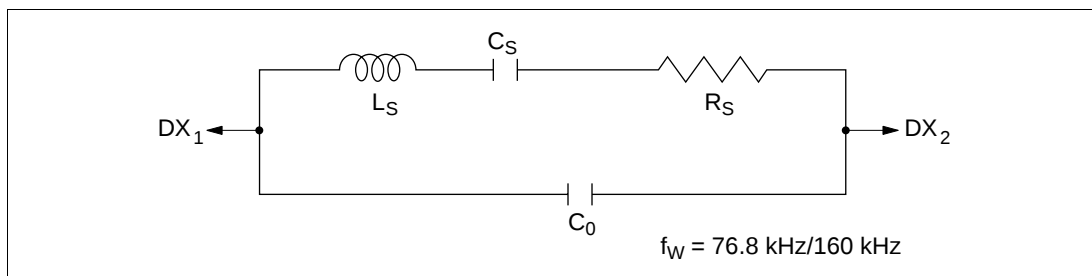
Figure 4-8 Equivalent Circuit of 76.8-kHz/160-kHz Crystal Oscillator
