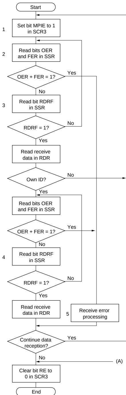
Figure 10-21 Example of Multiprocessor Data Reception Flowchart
