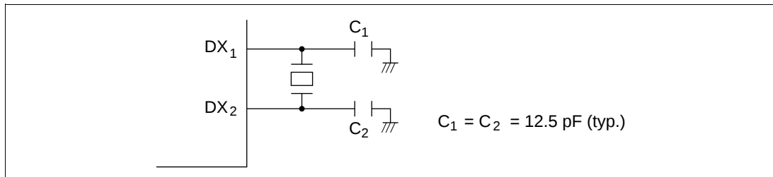
Figure 4-7 Typical Connection to 76.8-kHz/160-kHz Crystal Oscillator (Subclock)
