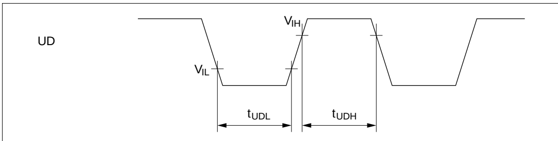
Figure 13-4 UD Pin Minimum Modulation Width Timing
