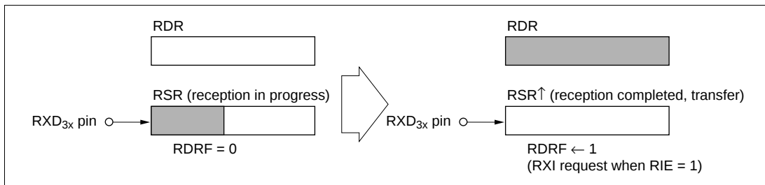
Figure 10-4 (a) RDRF Setting and RXI Interrupt
