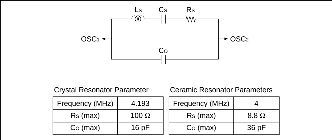
Figure 13-8 Resonator Equivalent Circuit
