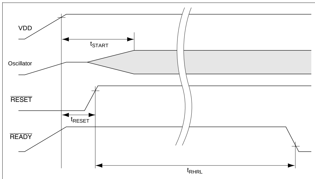
Figure 12-14 Start-up Timing
