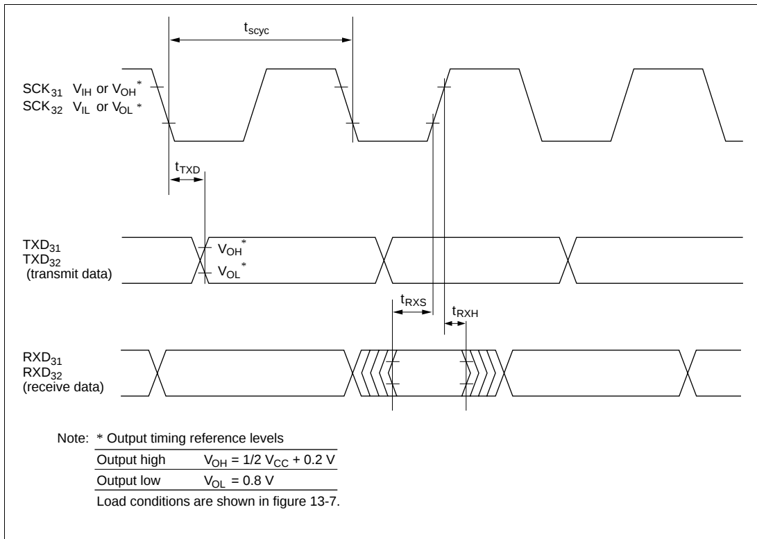
Figure 13-6 SCI3 Synchronous Mode Input/Output Timing
