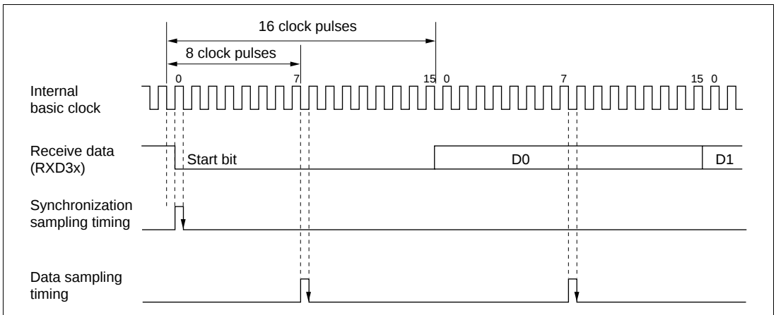
Figure 10-23 Receive Data Sampling Timing in Asynchronous Mode
