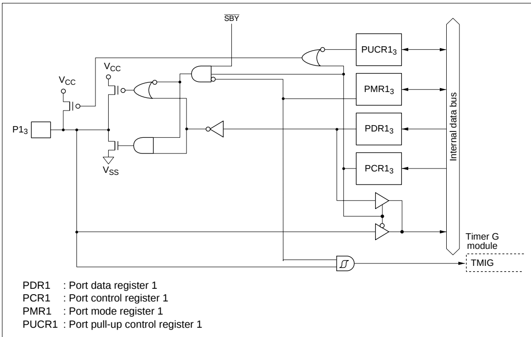
Figure C-1 (b) Port 1 Block Diagram (Pin P1 3 )
