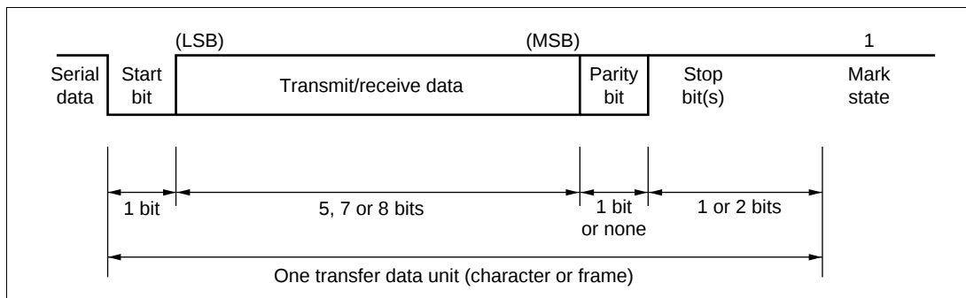
Figure 10-5 Data Format in Asynchronous Communication
