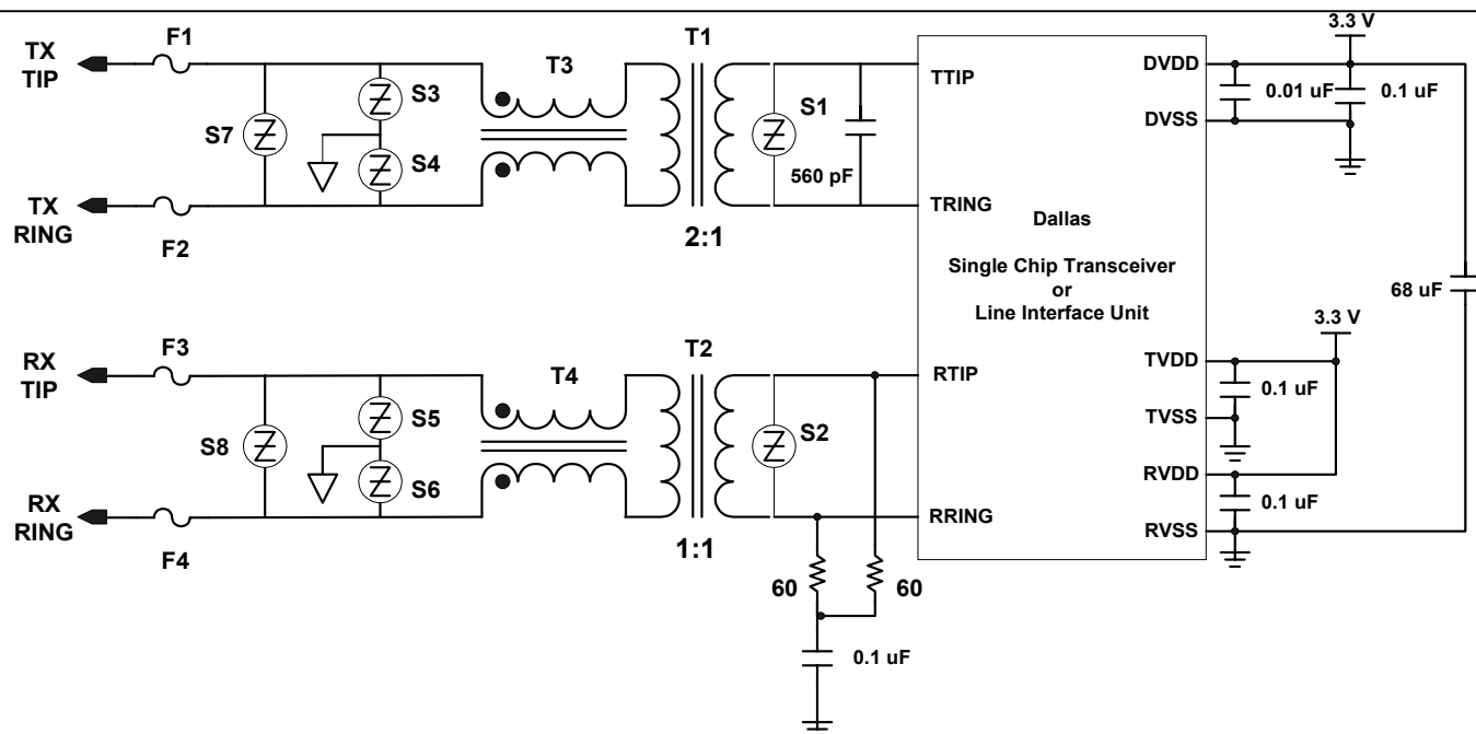
Figure 8-11. Basic Balanced Network Connections
