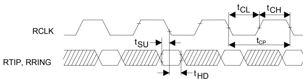
Figure 12-7. Receive Framing Timing—Line Side
