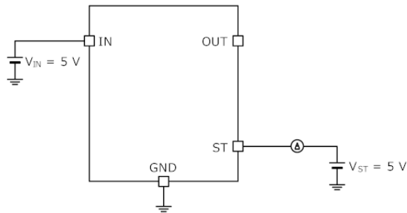
Measurement Circuit for Figure 20
