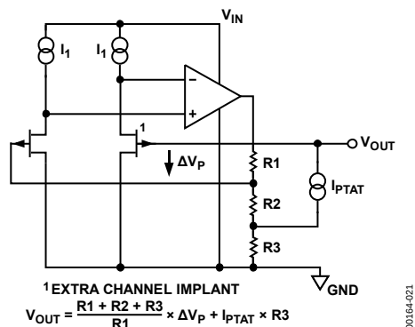
Figure 21. Simplified Schematic
