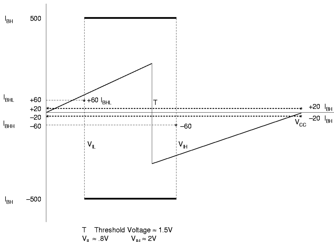
Figure 2: Trip and Hold Current Characteristics of the Last Valve Latch
