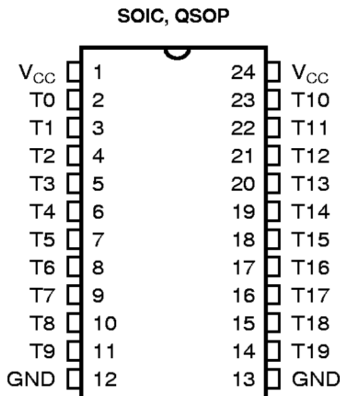
Figure 2. Pin Configuration (All Pins Top View)
