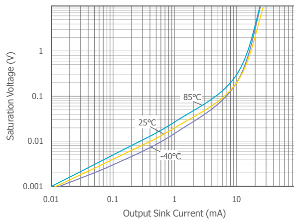
Output Sink Current vs. Saturation Voltage (CLC4550)
