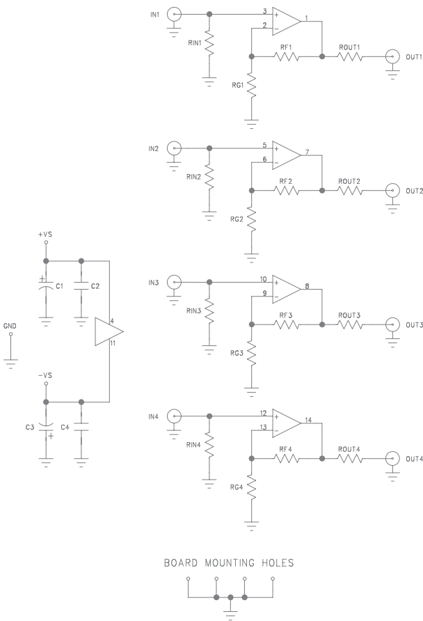
Figure 12. CEB018 Schematic
