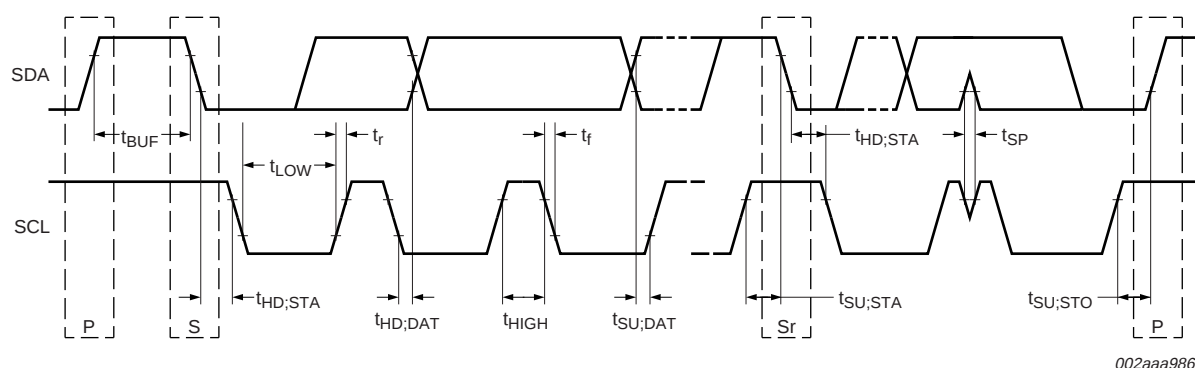
Fig 19. Definition of timing
