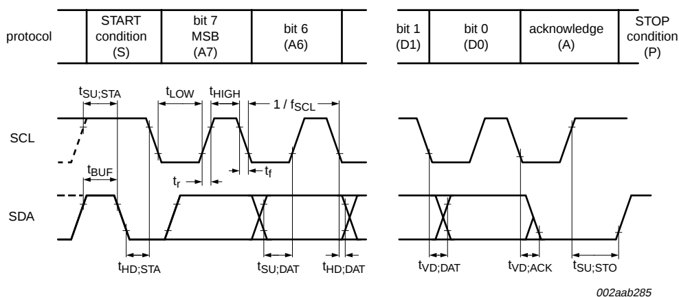
Fig 20. I 2 C-bus timing diagram
