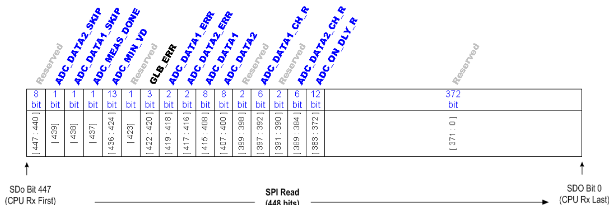
Figure 6 - DTC (Duty-Cycle) Write / Read SPI Communication Packets
