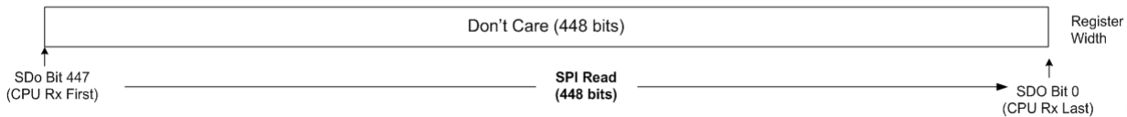
Figure 12 - DTC (Duty-Cycle) Read SPI Communication Packets
